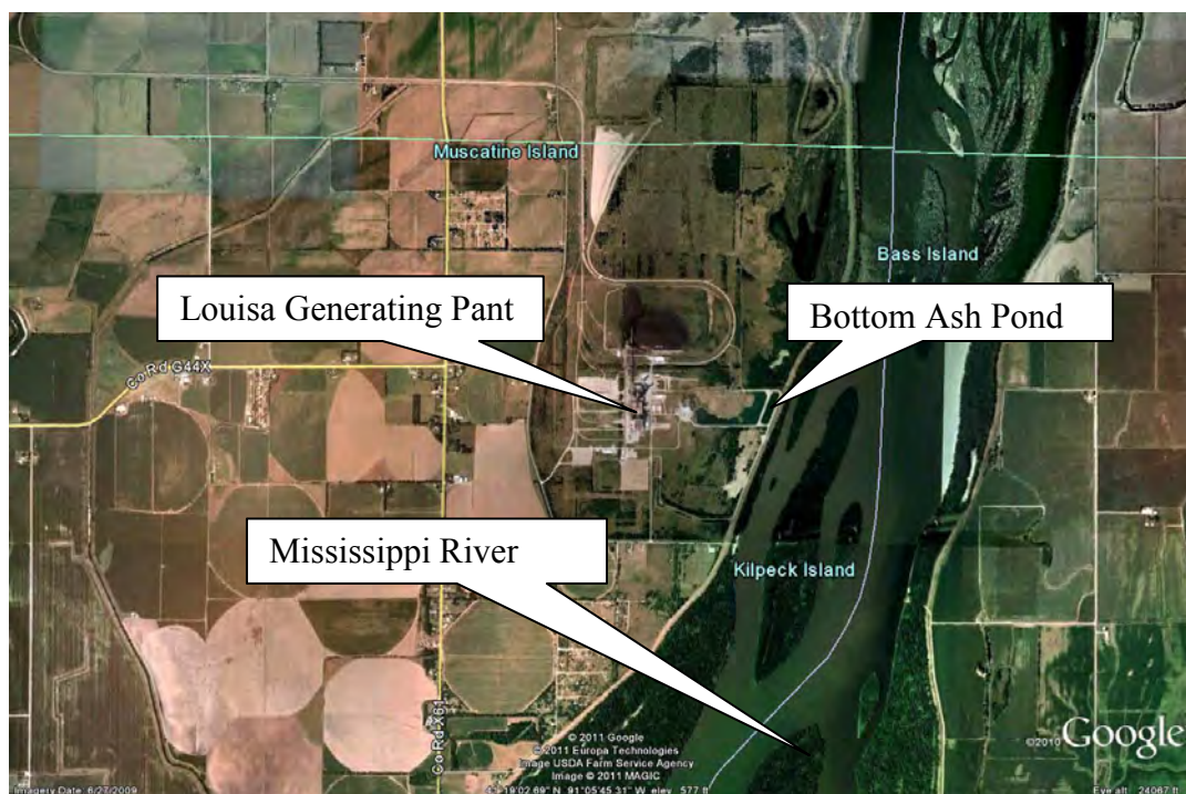
Figure 2.1b: Louisa Generating Plant Aerial Photograph.
