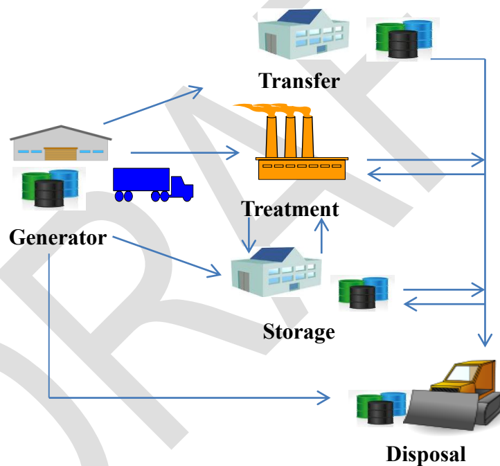
FIGURE 1-4: Waste Analysis Data Flow
