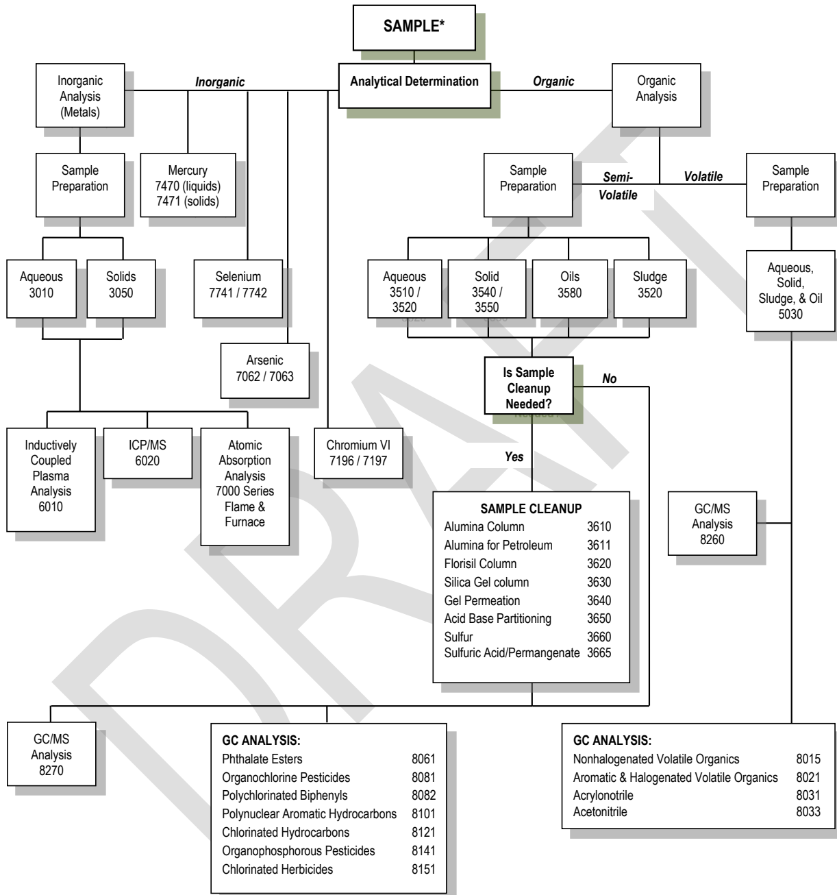
FIGURE 2-7: Analytical Methods Selection Flowchart
