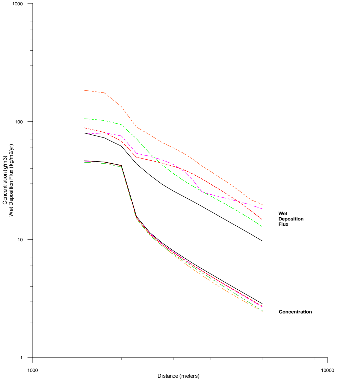
3000m Ground-Level Area Source (LAU) 2 Particle Sizes Met Station: Tucson _____ No SCIM - - - - - SCIM 25 Hours - - - - - SCIM 49 Hours - - - - - SCIM 97 Hours - - - - - SCIM 193 Hours
