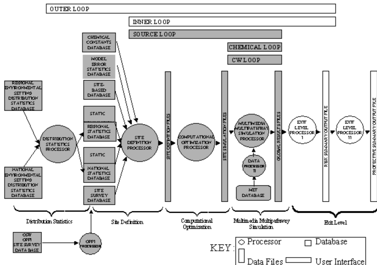
Figure 8.18 View of the Exit Level Processors
