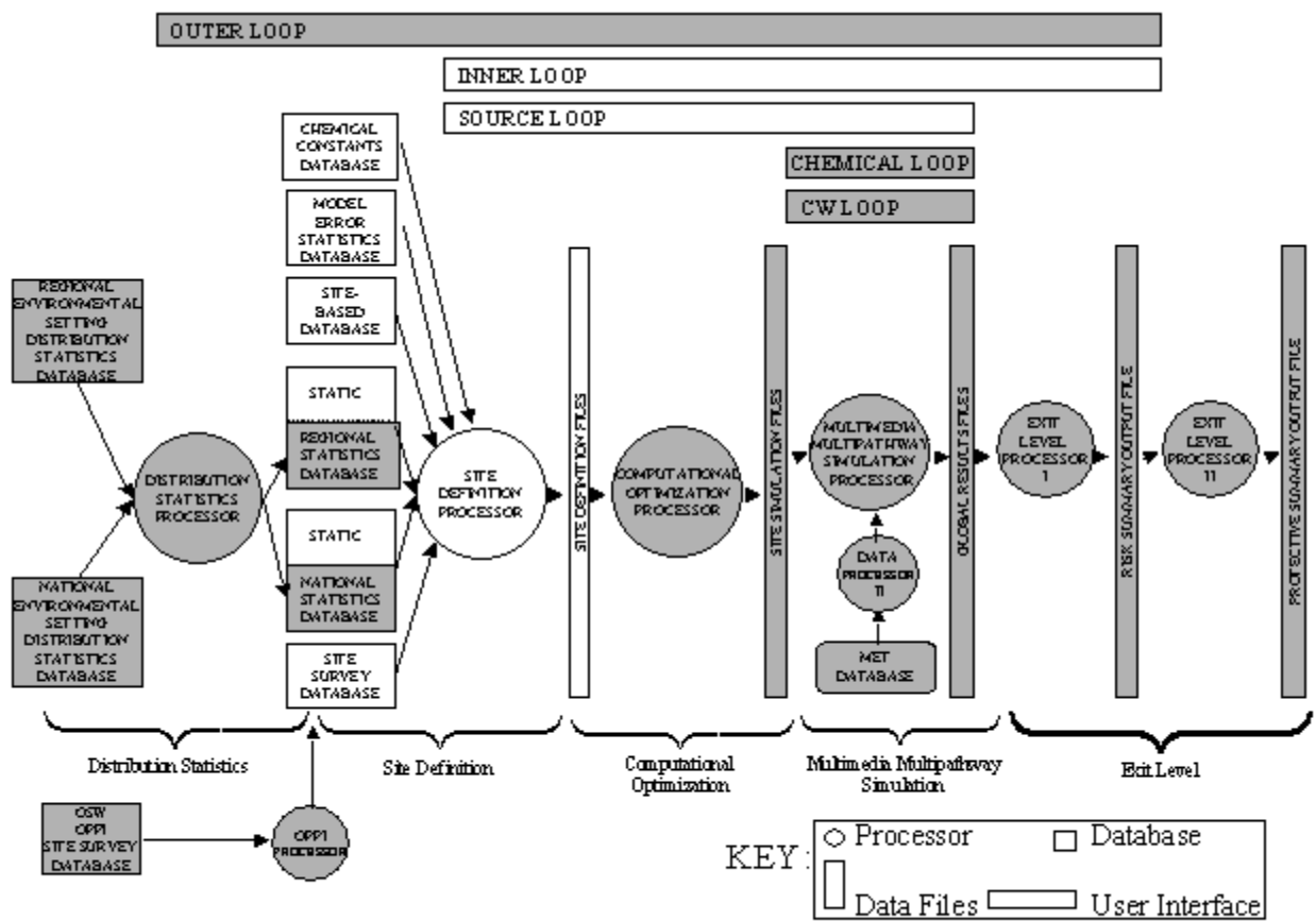
Figure 8.13 View of the Site Definition Processor
