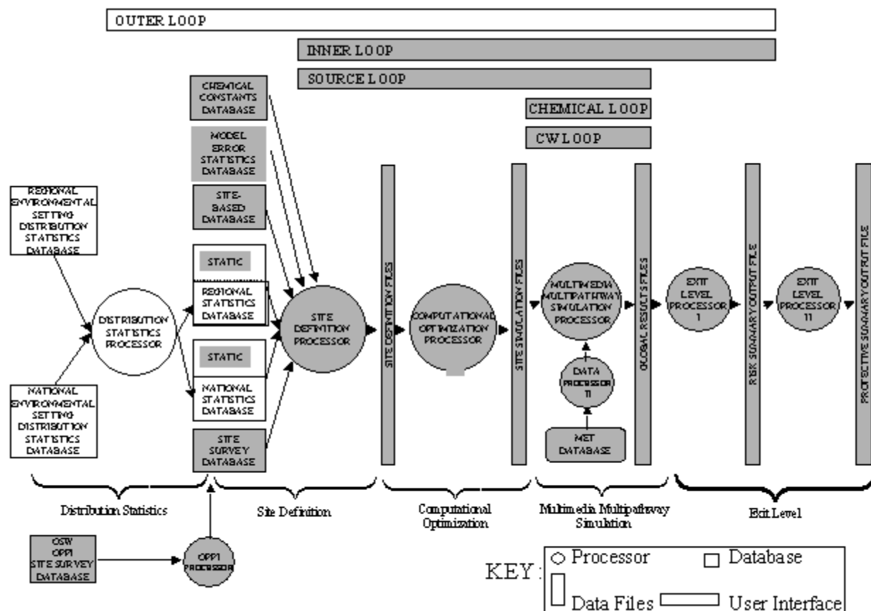
Figure 8.12 View of the Distribution Statistics Processor
