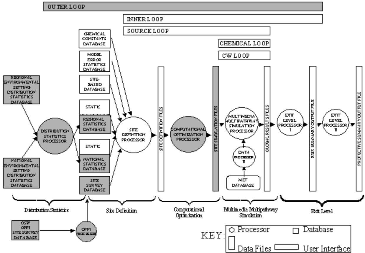
Figure 8.11 Overall Diagram of the Protocols for Implementing a Two-Stage Monte Carlo Analysis
