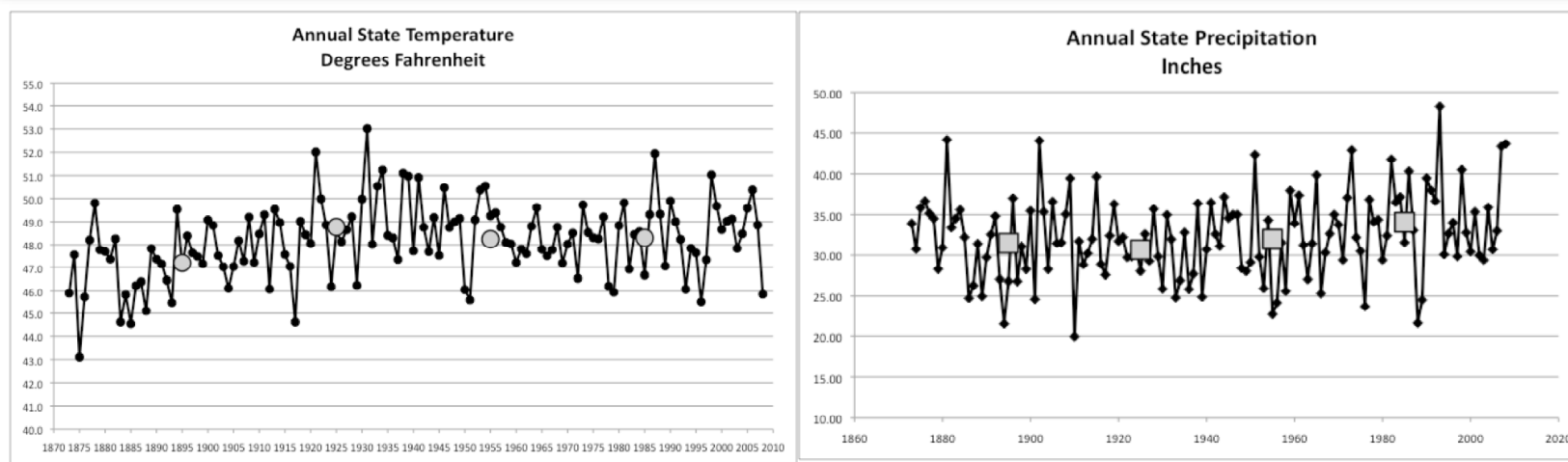
Figure 3. Statewide annual temperature and precipitation computed from State Climatologist 33-station data set. Grey-shaded boxes are 30-year average for 1881-1910, 1911-1940, 1941-1970, and 1971-2000.
