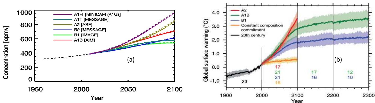
Figure 1. (a) Carbon dioxide concentration of global greenhouse gas emissions scenarios ( http://www.ipcc-data.org/ddc_co2.html ). (b) Average and range (shown by shading) of global temperature change simulated by GCMs given emissions scenarios for the 21 st century.
