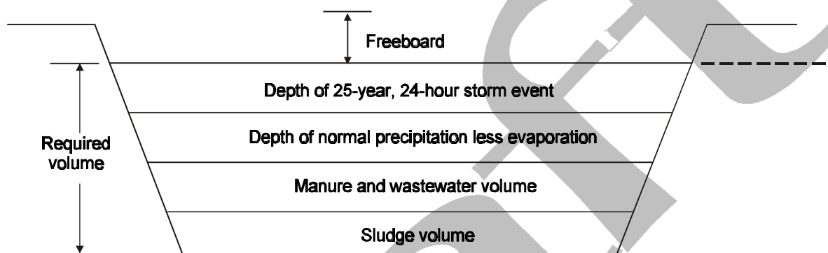
Figure 1 Cross Section of Animal Waste Storage Pond
