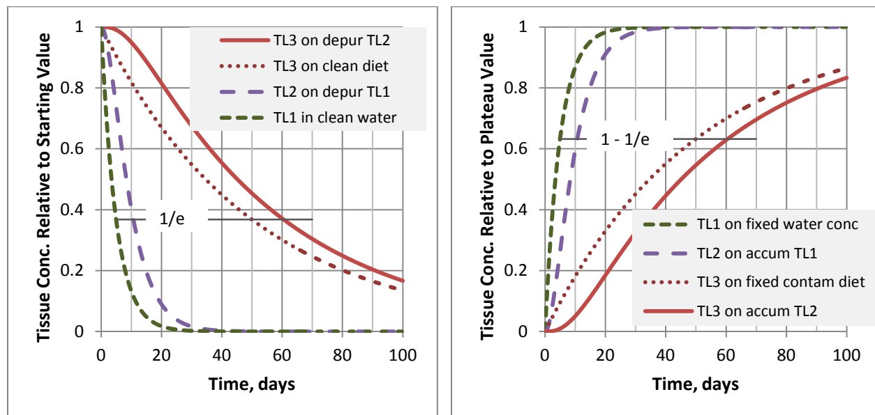
Figures J1 a & b. Depuration and accumulation behavior for algae-detritus-sediment k=0.2/\text{day} , invertebrate k=0.2/\text{day} and fish k=0.02/\text{day} , calculated with time step = 0.1 day. Concentration is expressed as a dimensionless ratio: concentration at time t divided by either starting concentration (J1a) or plateau concentration (J1b).
