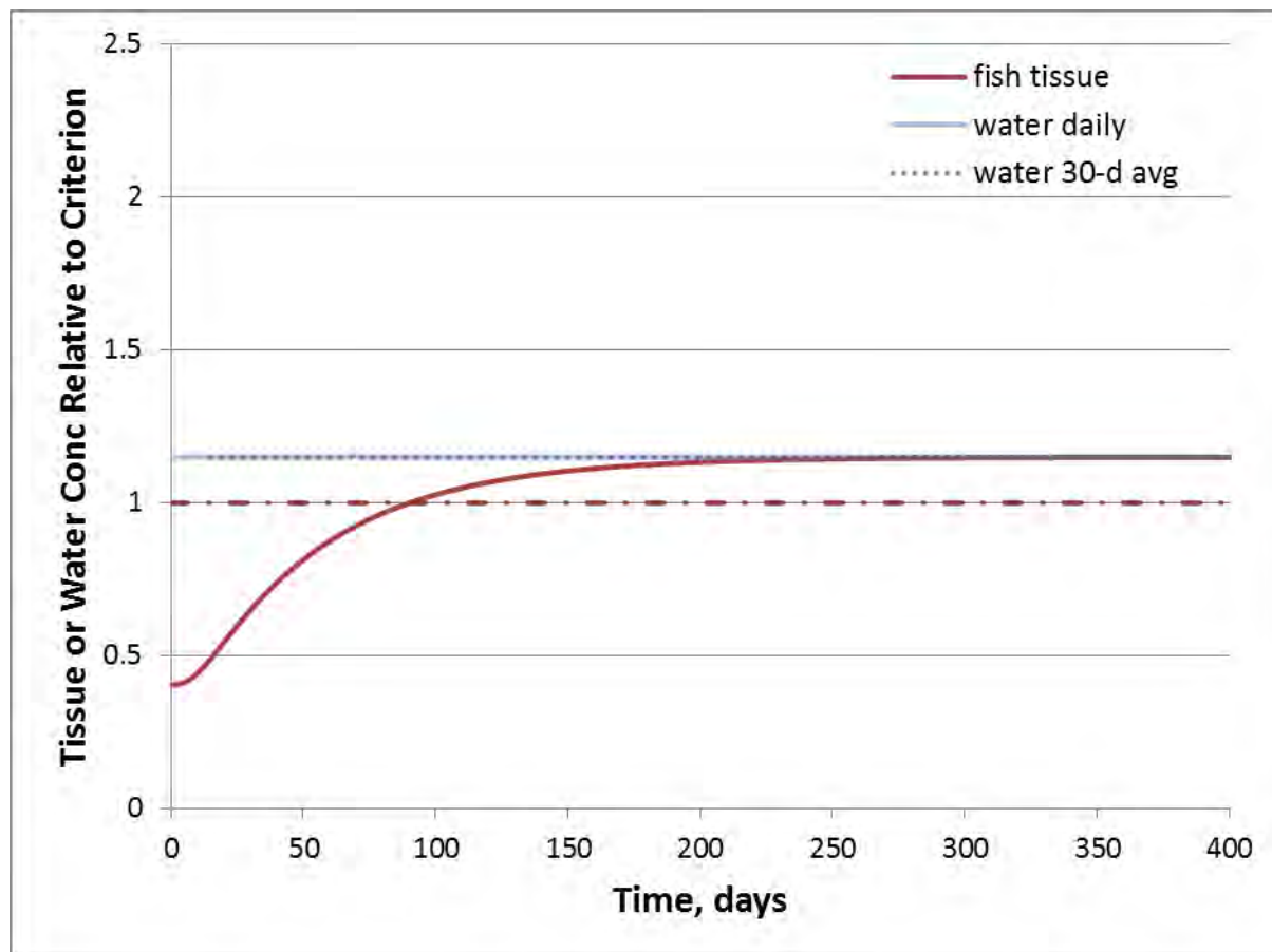
Figure J4. TL3 concentration responding to a Time=0 step-function increase in water concentration that remains time-invariant thereafter. Given that the water concentration is too high, ultimately yielding tissue concentrations at the hypothetical sensitive species EC20, 1.15-fold above the criterion, and given the previously presented kinetic parameters, it is calculated to take 90 days for TL3 concentrations to rise above the criterion.
