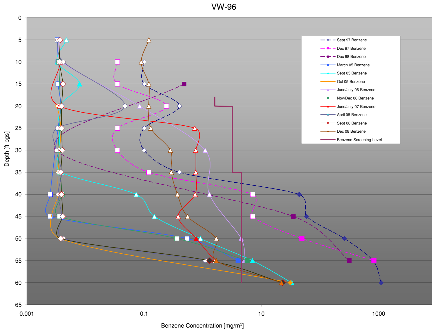
FIGURE 3-24b. BENZENE PROFILE, NESTED VAPOR MONITORING WELL VW-96 SECOND 2008 SEMIANNUAL MONITORING EVENT CHEVRON CINCINNATI FACILITY, HOOVEN, OHIO
