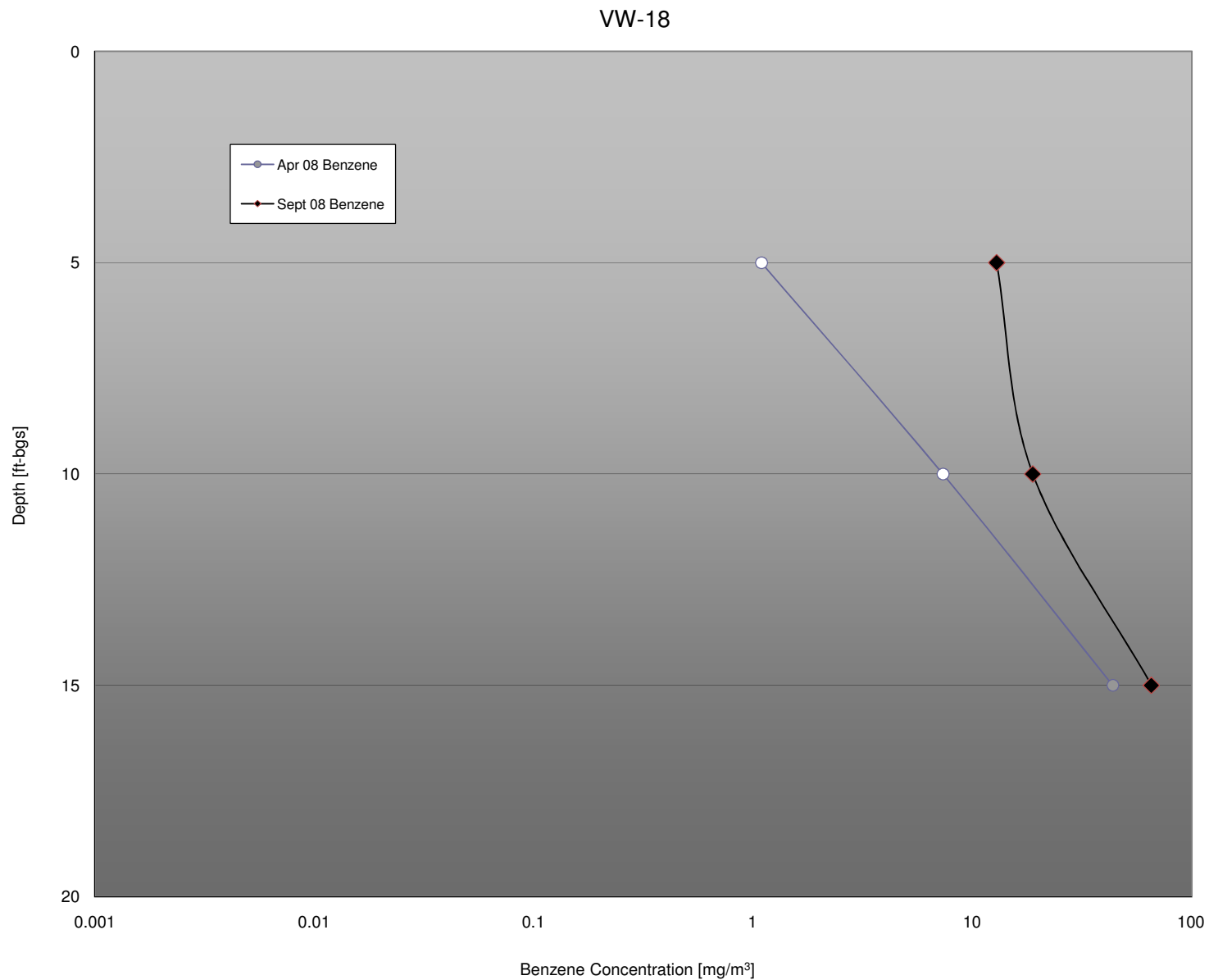
FIGURE 3-20b. BENZENE PROFILE, NESTED VAPOR MONITORING WELL VW-18 SECOND 2008 SEMI-ANNUAL MONITORING EVENT CHEVRON CINCINNATI FACILITY, HOOVEN, OHIO
