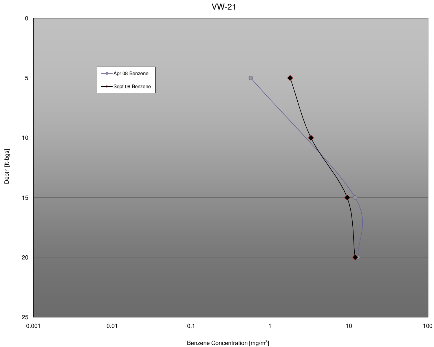
FIGURE 3-21b. BENZENE PROFILE, NESTED VAPOR MONITORING WELL VW-21 SECOND 2008 SEMIANNUAL MONITORING EVENT CHEVRON CINCINNATI FACILITY, HOOVEN, OHIO
