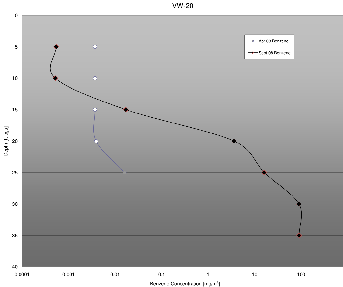
FIGURE 3-22b. BENZENE PROFILE, NESTED VAPOR MONITORING WELL VW-20 SECOND 2008 SEMIANNUAL MONITORING EVENT CHEVRON CINCINNATI FACILITY, HOOVEN, OHIO
