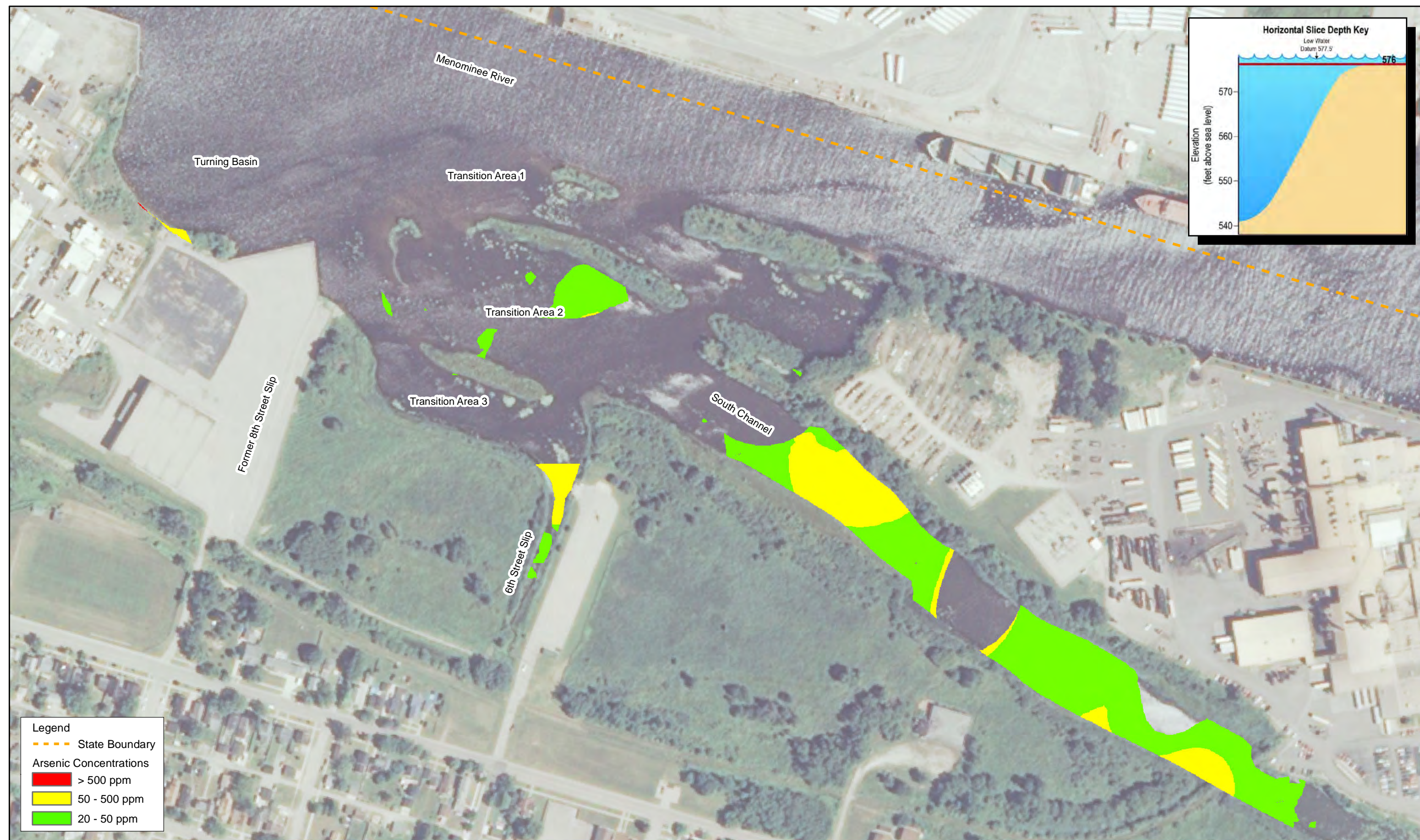
Figure 15P Horizontal Slice of Project Area, Arsenic Concentrations Elevation 576' Tyco Fire Products LP Facility Marinette, WI
