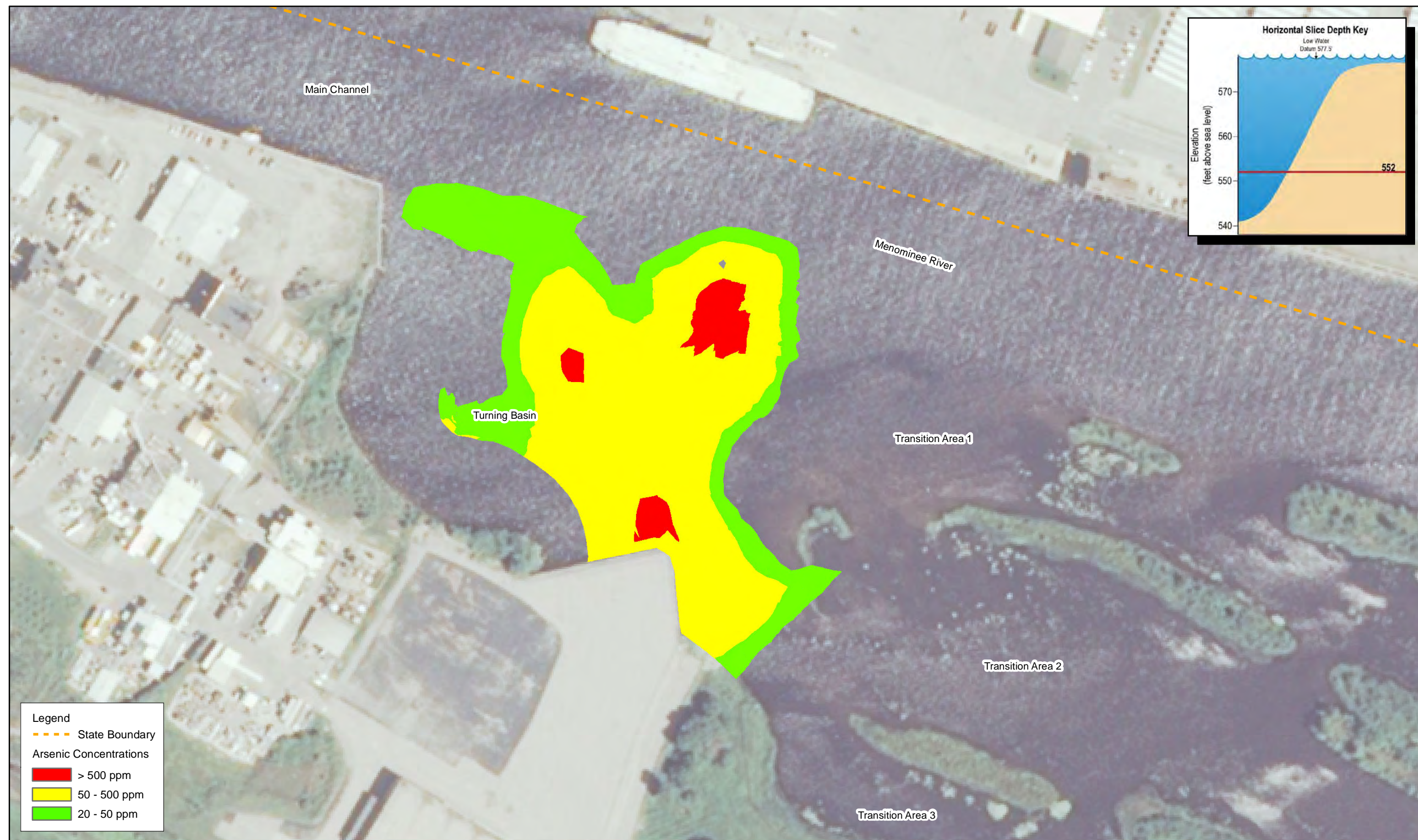
Figure 15D Horizontal Slice of Project Area, Arsenic Concentrations Elevation 552' Tyco Fire Products LP Facility Marinette, WI
