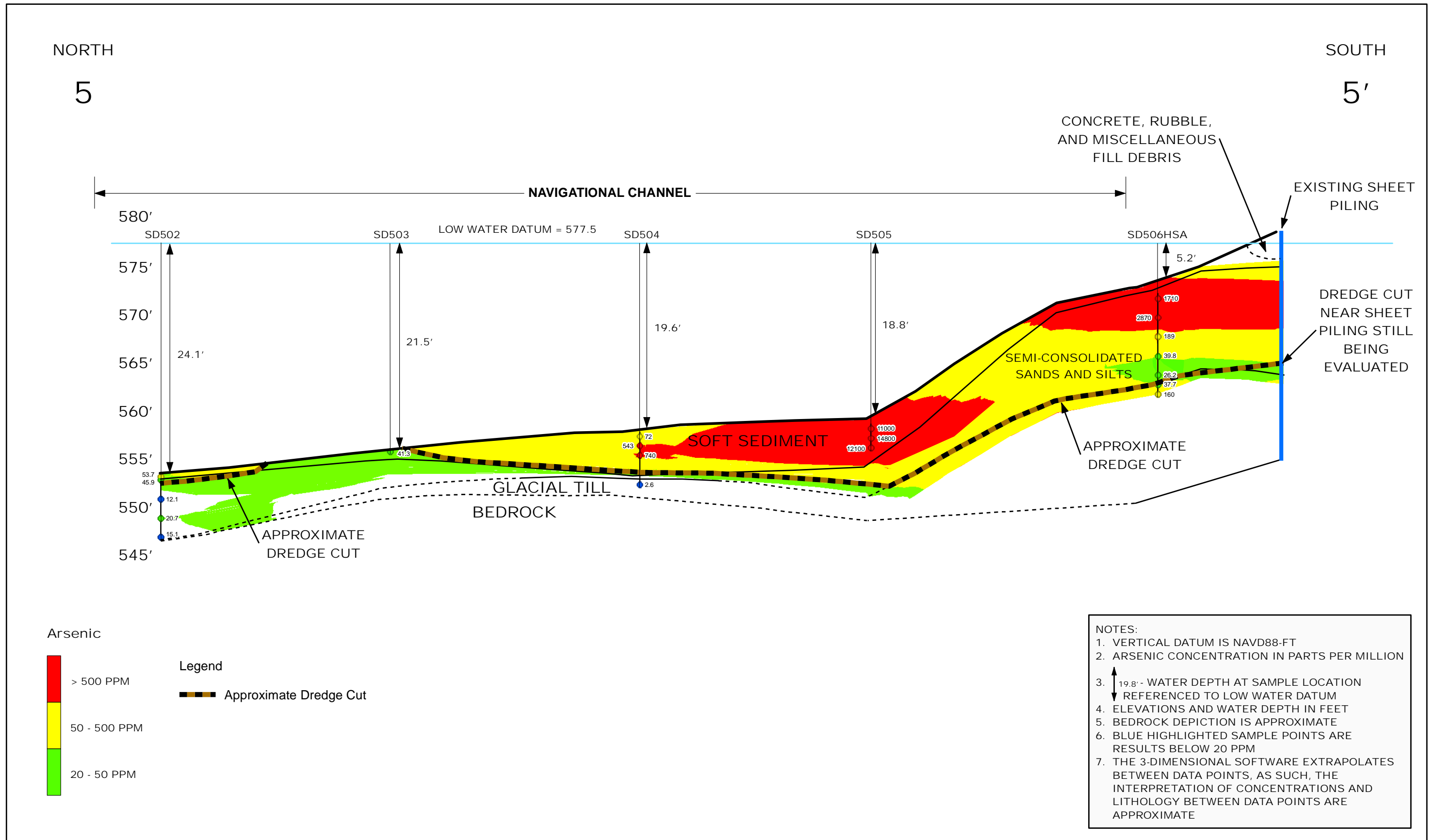
Figure 17E Cross-section 5-5' Tyco Fire Products LP Facility Marinette, WI
