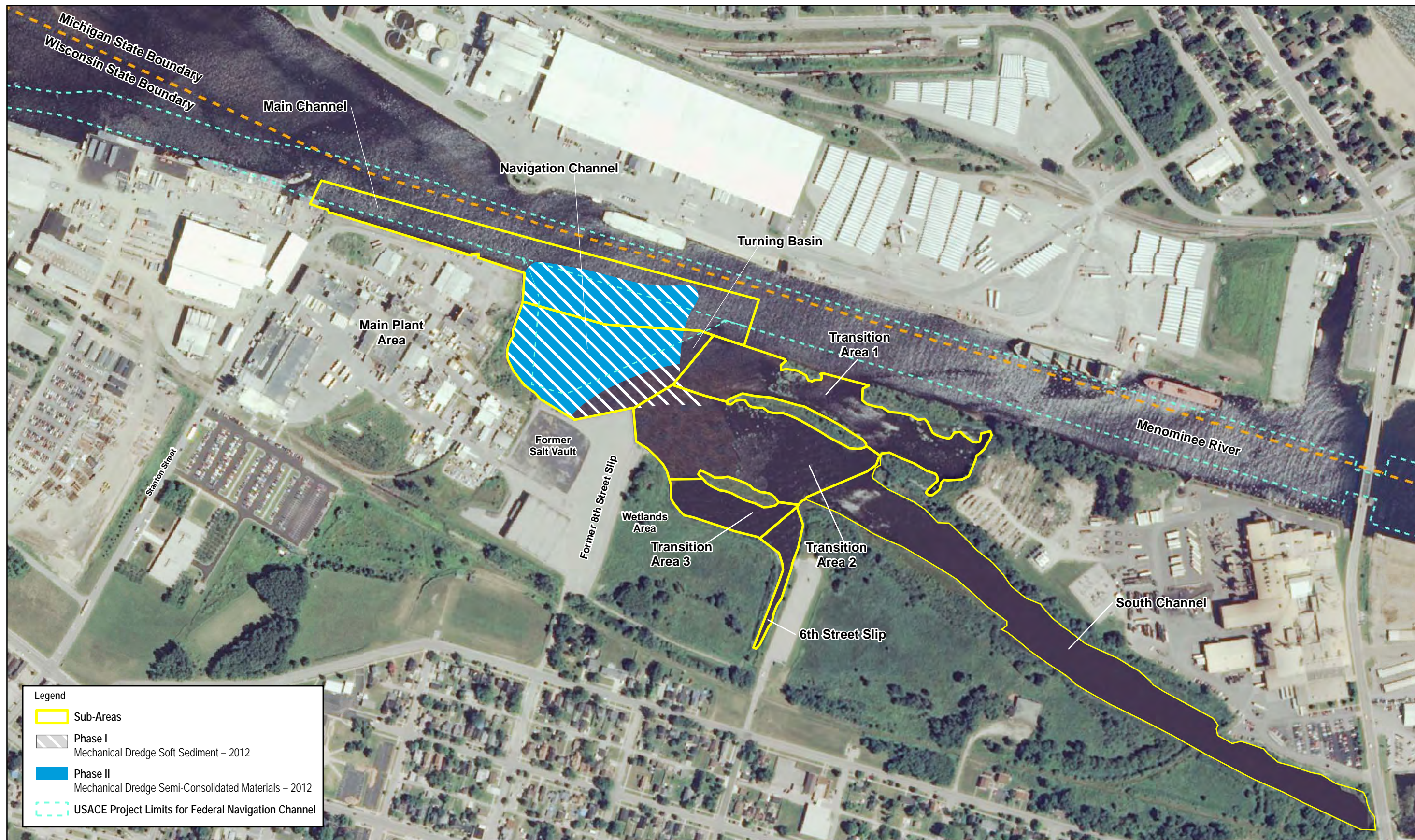
FIGURE 18A Remediation Sequence 2012 Tyco Fire Products Facility Marinette, WI
