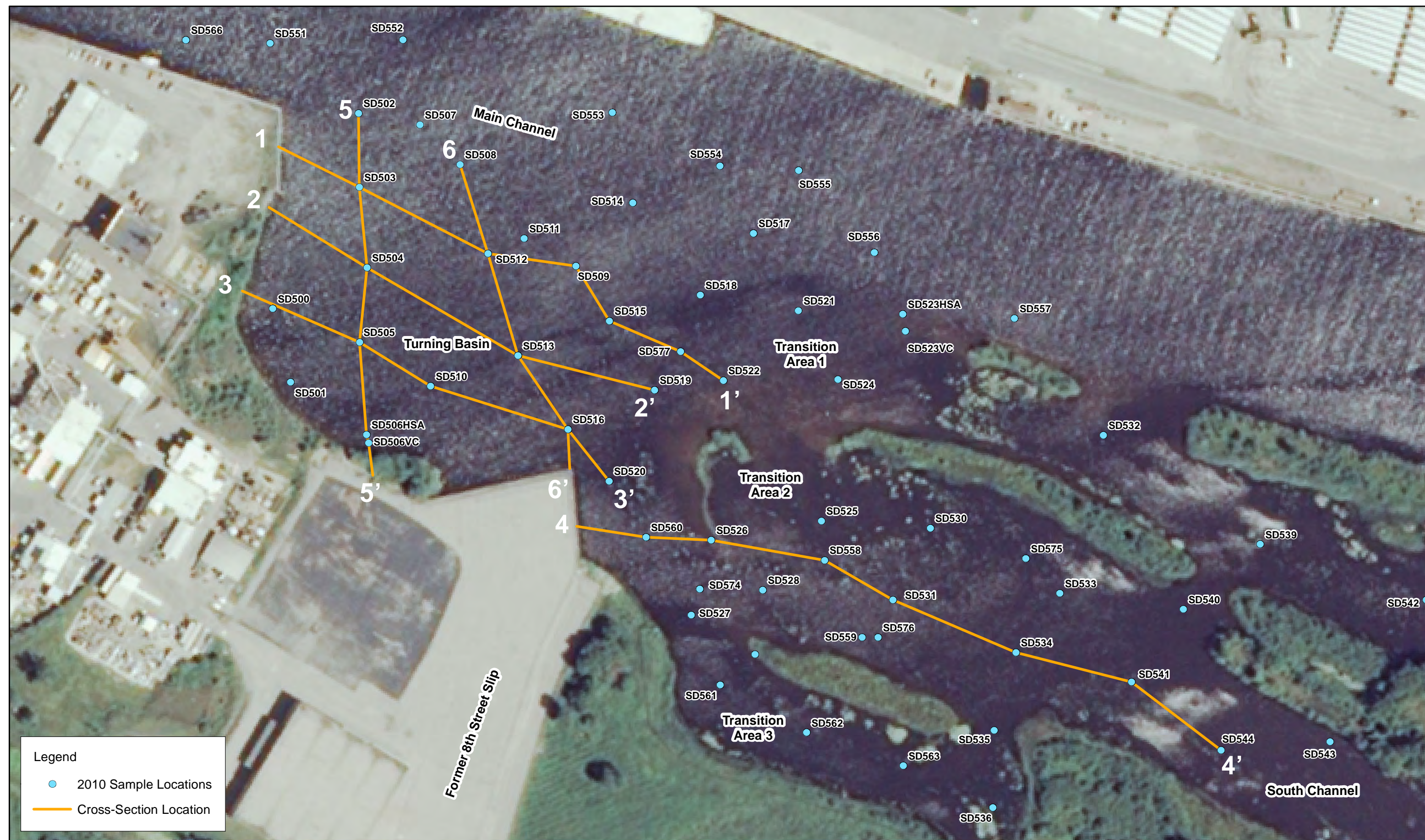
Figure 16 Cross-Section Location Tyco Fire Products LP Facility Marinette, WI
