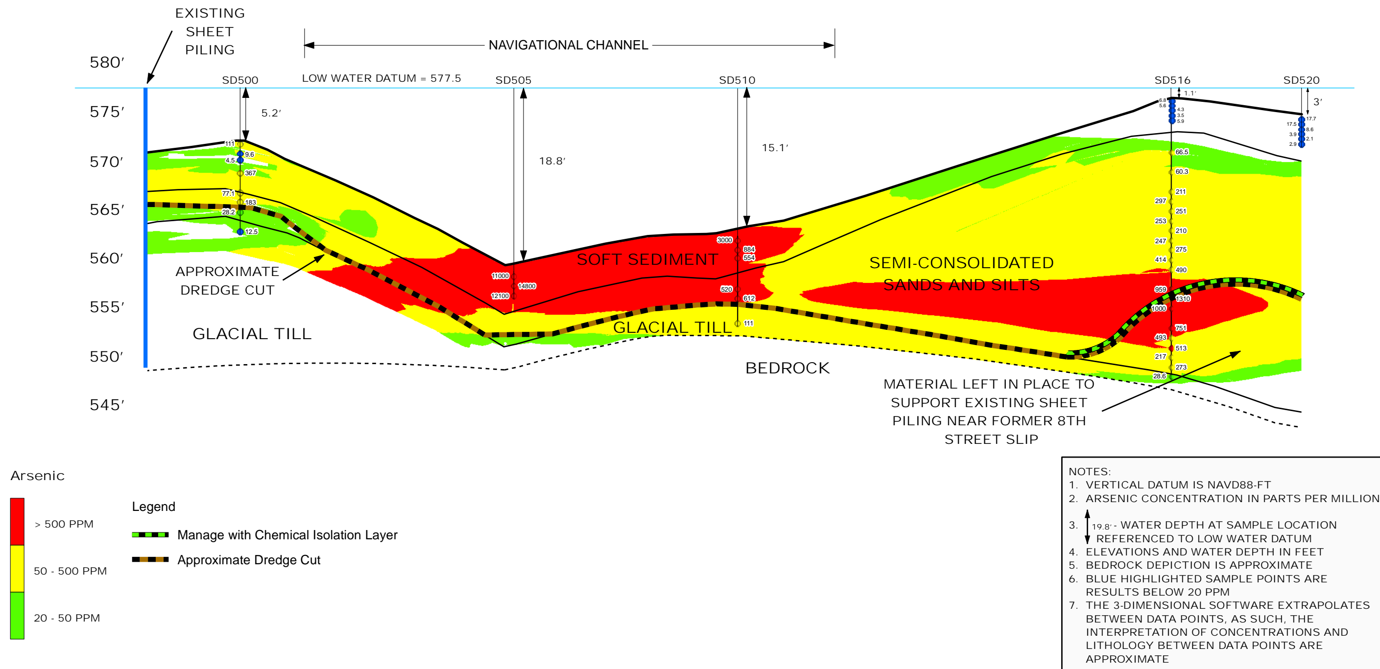
Figure 17C Cross-section 3-3' Tyco Fire Products LP Facility Marinette, WI
