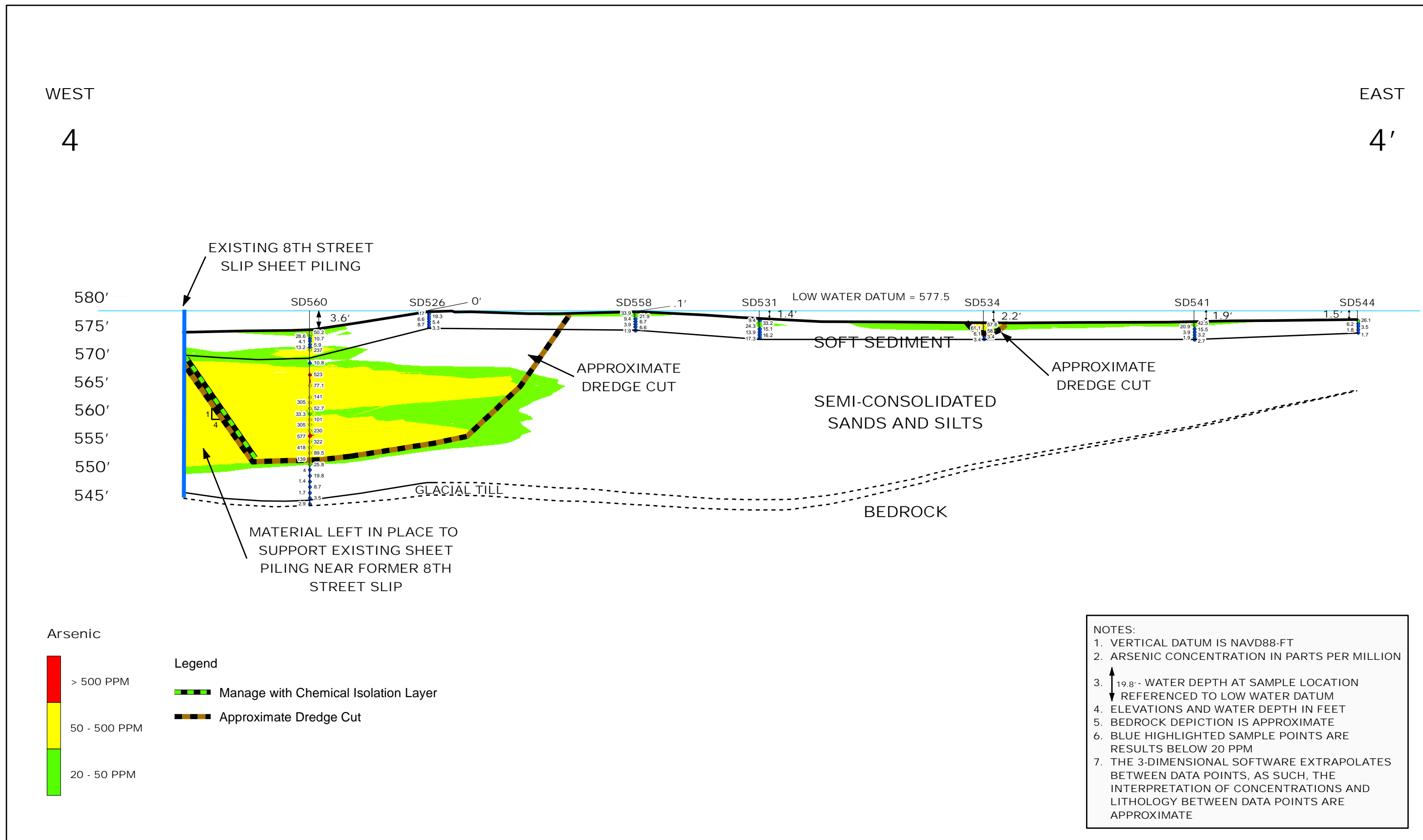
Figure 17D Cross-section 4-4' Tyco Fire Products LP Facility Marinette, WI
