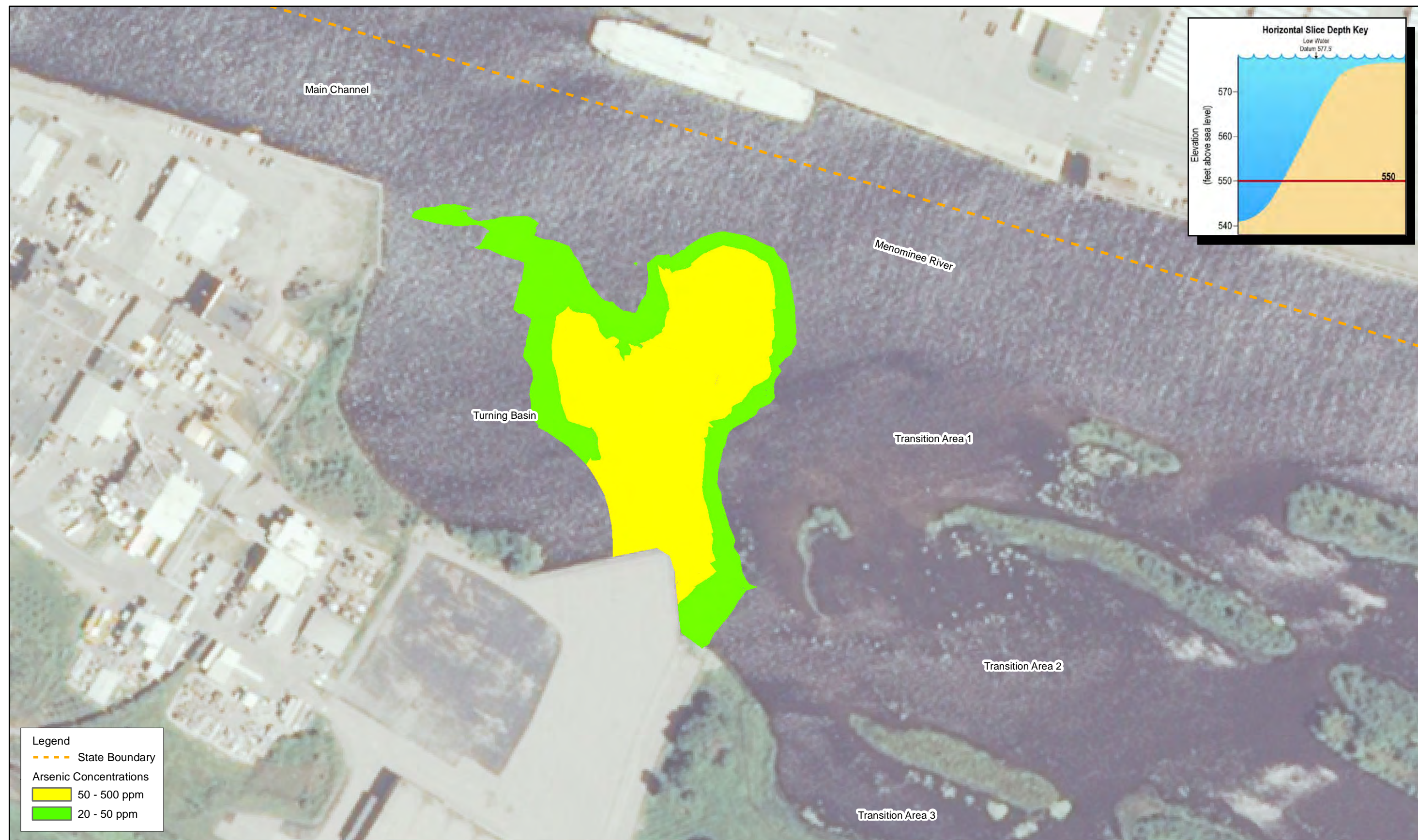
Figure 15C Horizontal Slice of Project Area, Arsenic Concentrations Elevation 550' Tyco Fire Products LP Facility Marinette, WI
