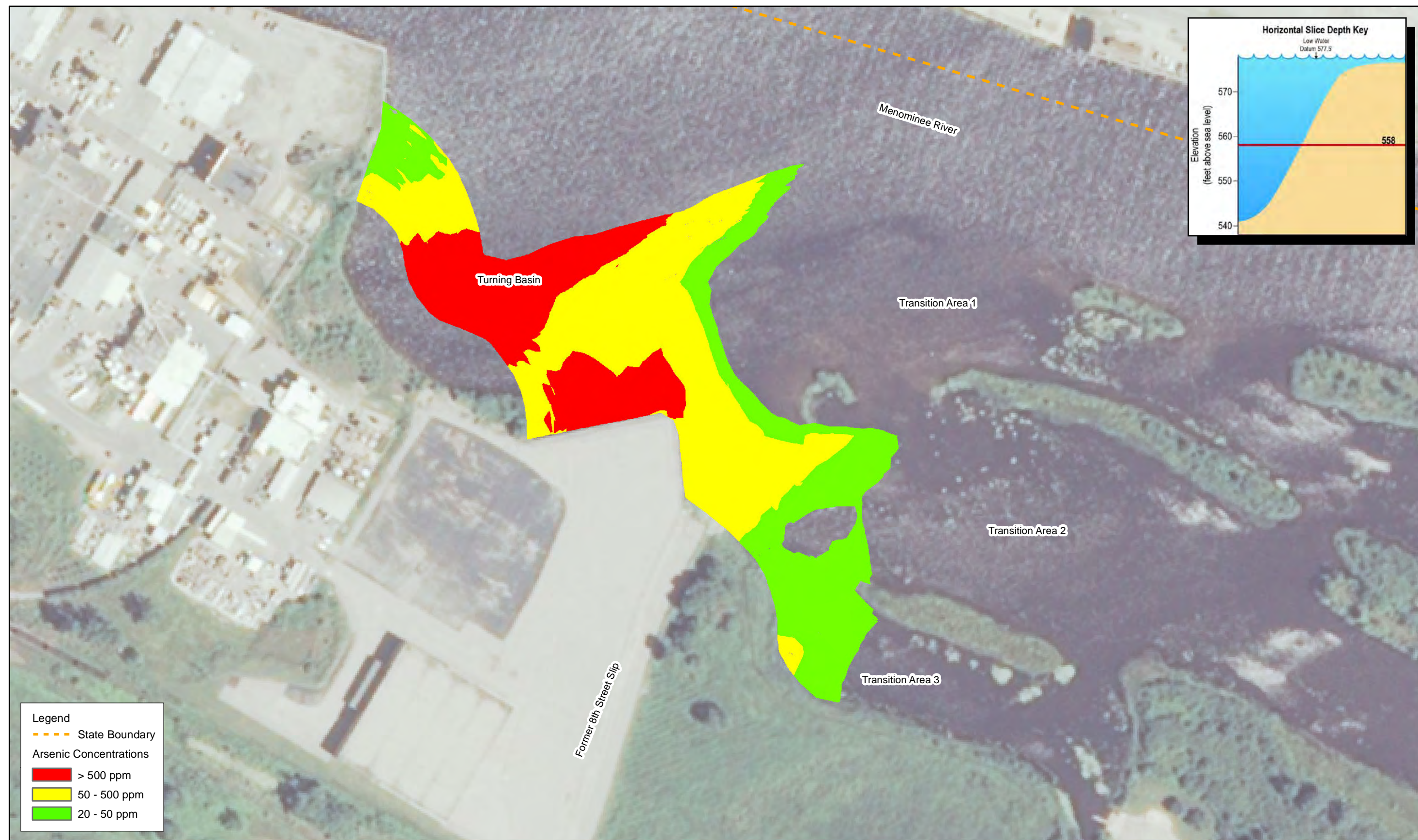
Figure 15G Horizontal Slice of Project Area, Arsenic Concentrations Elevation 558' Tyco Fire Products LP Facility Marinette, WI
