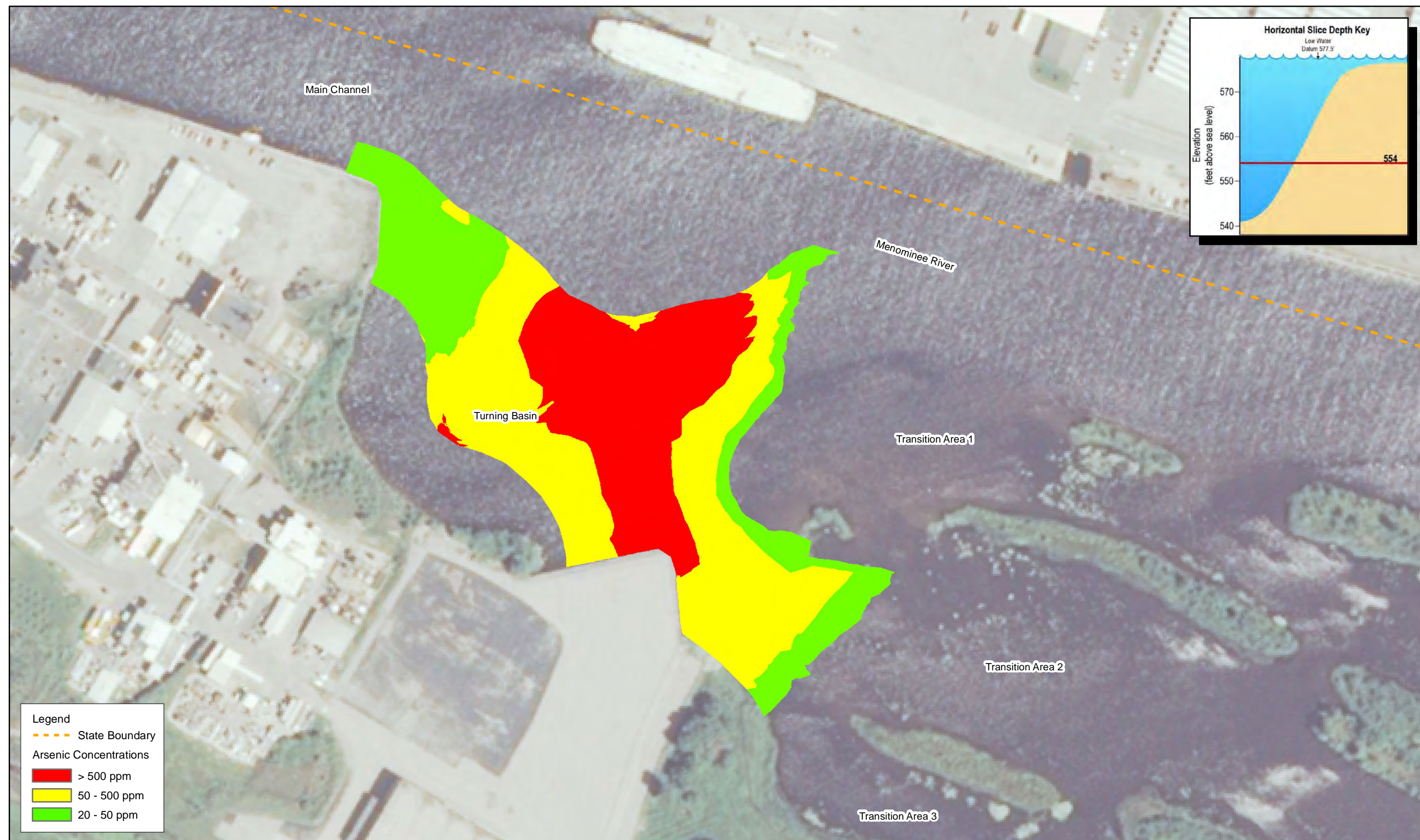
Figure 15E Horizontal Slice of Project Area, Arsenic Concentrations Elevation 554' Tyco Fire Products LP Facility Marinette, WI
