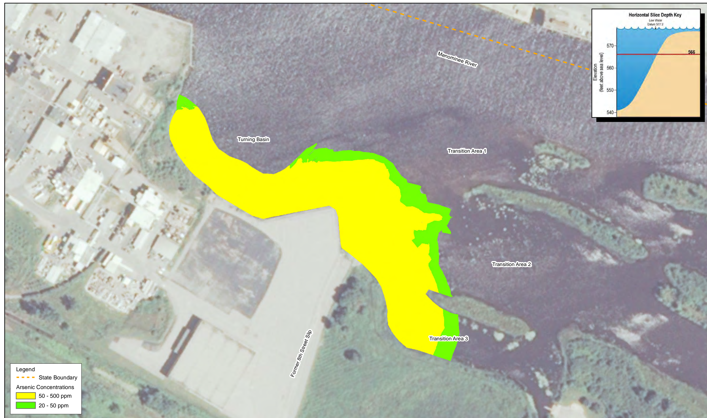
Figure 15K Horizontal Slice of Project Area, Arsenic Concentrations Elevation 566' Tyco Fire Products LP Facility Marinette, WI
