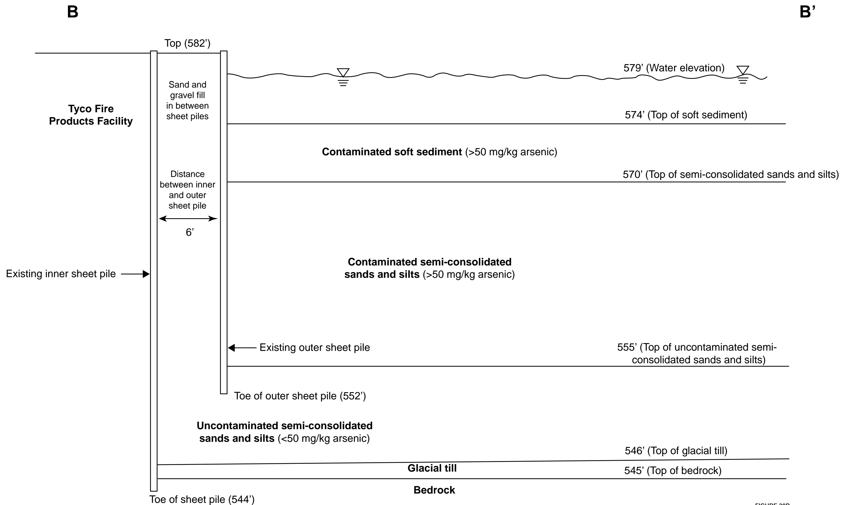
FIGURE 20B Sheet Piling Assessment Cross Section B-B' Tyco Fire Products Facility
