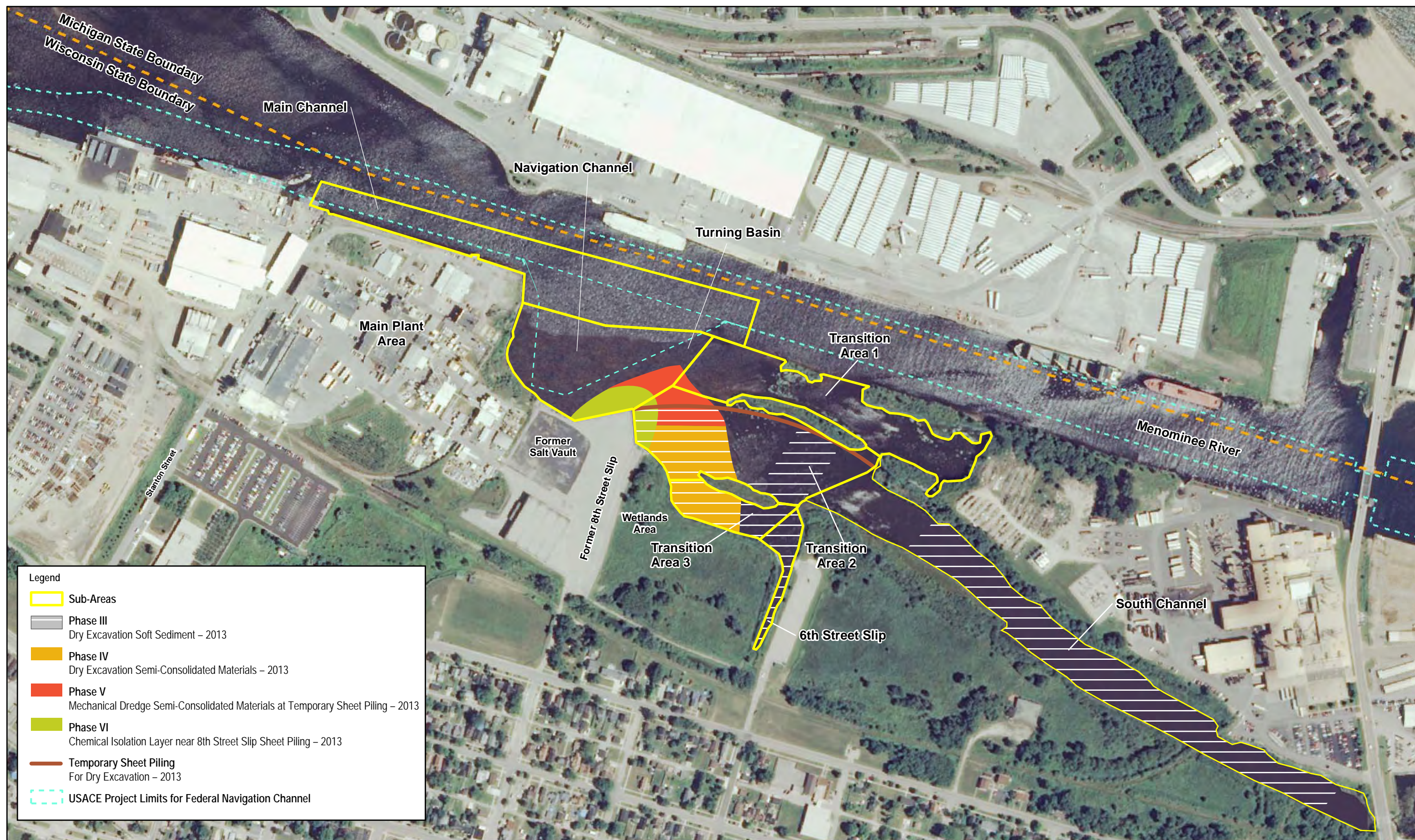
FIGURE 18B Remediation Sequence 2013 Tyco Fire Products Facility Marinette, WI
