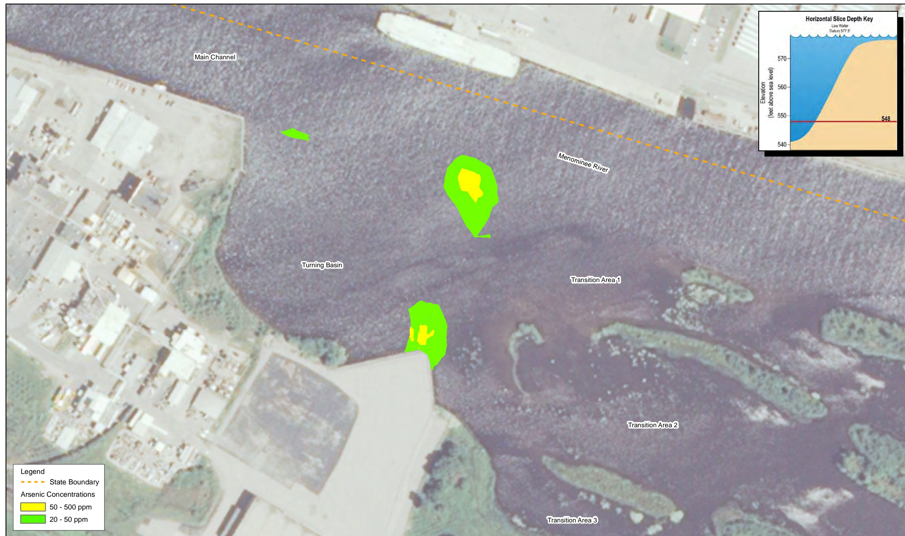
Figure 15B Horizontal Slice of Project Area, Arsenic Concentrations Elevation 548' Tyco Fire Products LP Facility Marinette, WI
