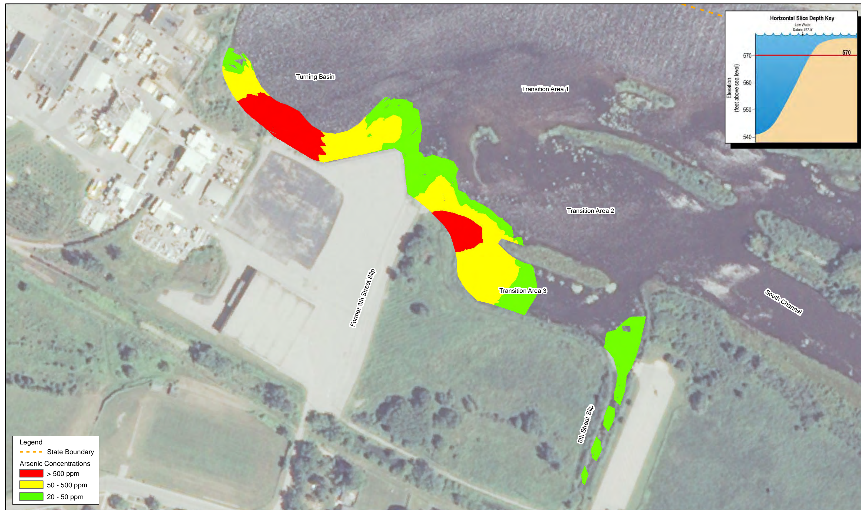
Figure 15M Horizontal Slice of Project Area, Arsenic Concentrations Elevation 570' Tyco Fire Products LP Facility Marinette, WI
