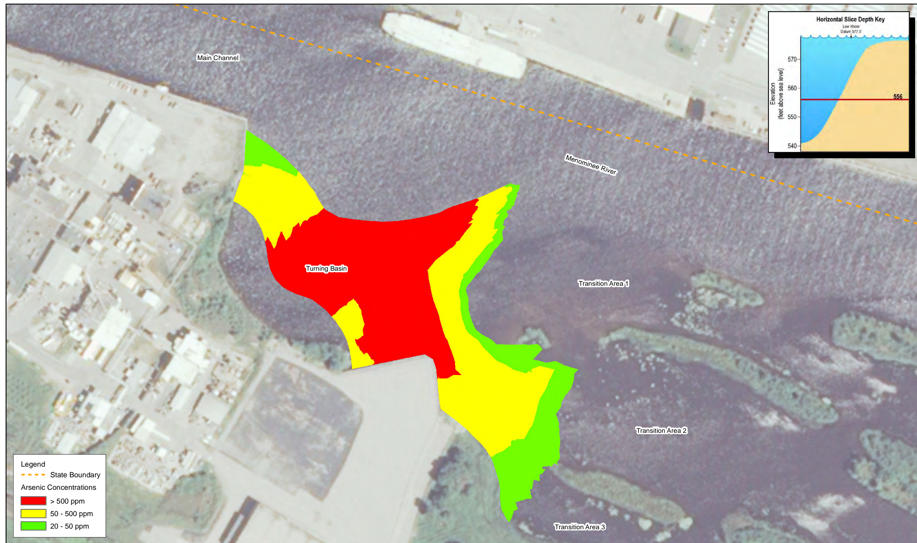
Figure 15F Horizontal Slice of Project Area, Arsenic Concentrations Elevation 556' Tyco Fire Products LP Facility Marinette, WI
