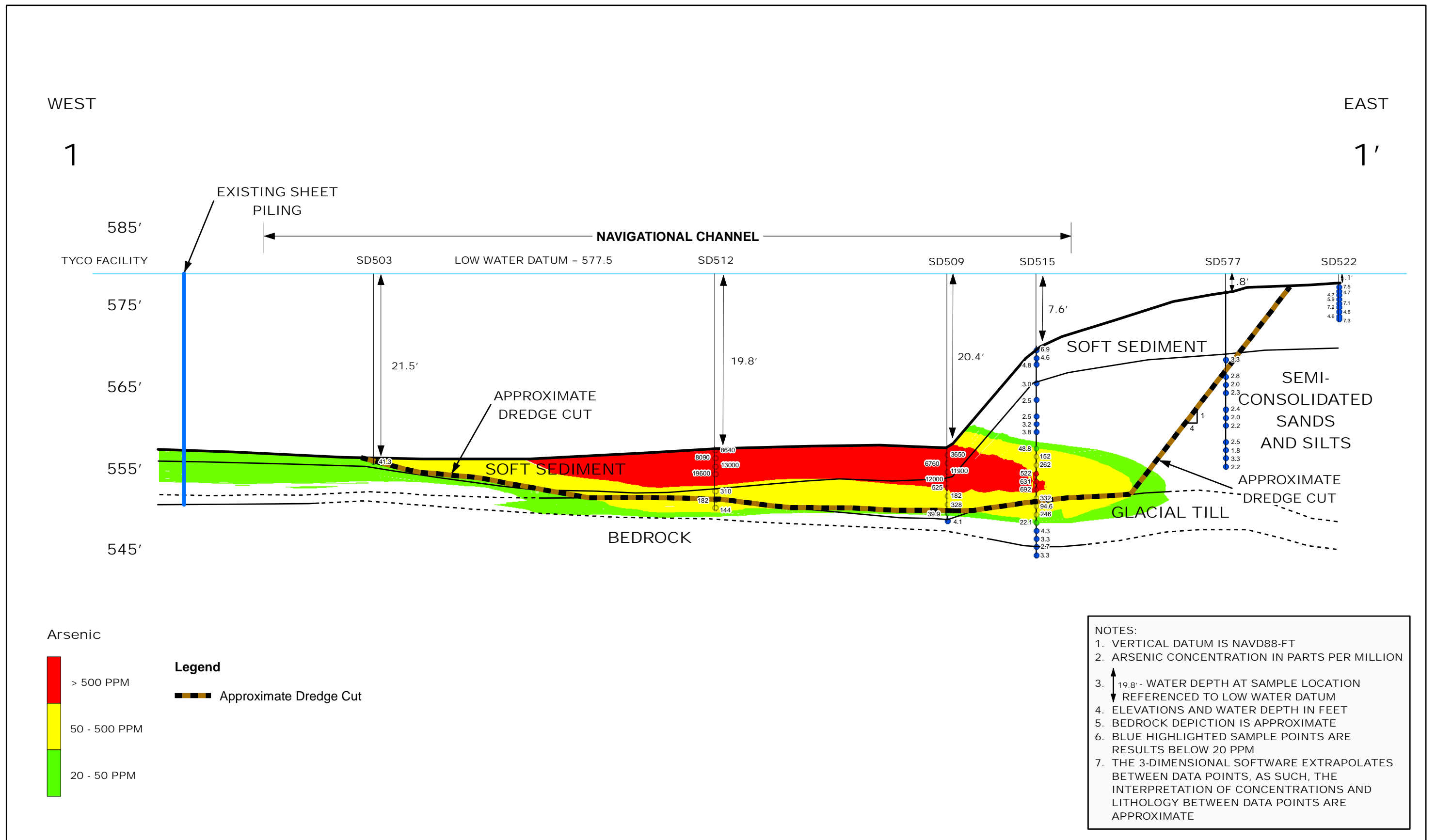
Figure 17A Cross-section 1-1' Tyco Fire Products LP Facility Marinette, WI
