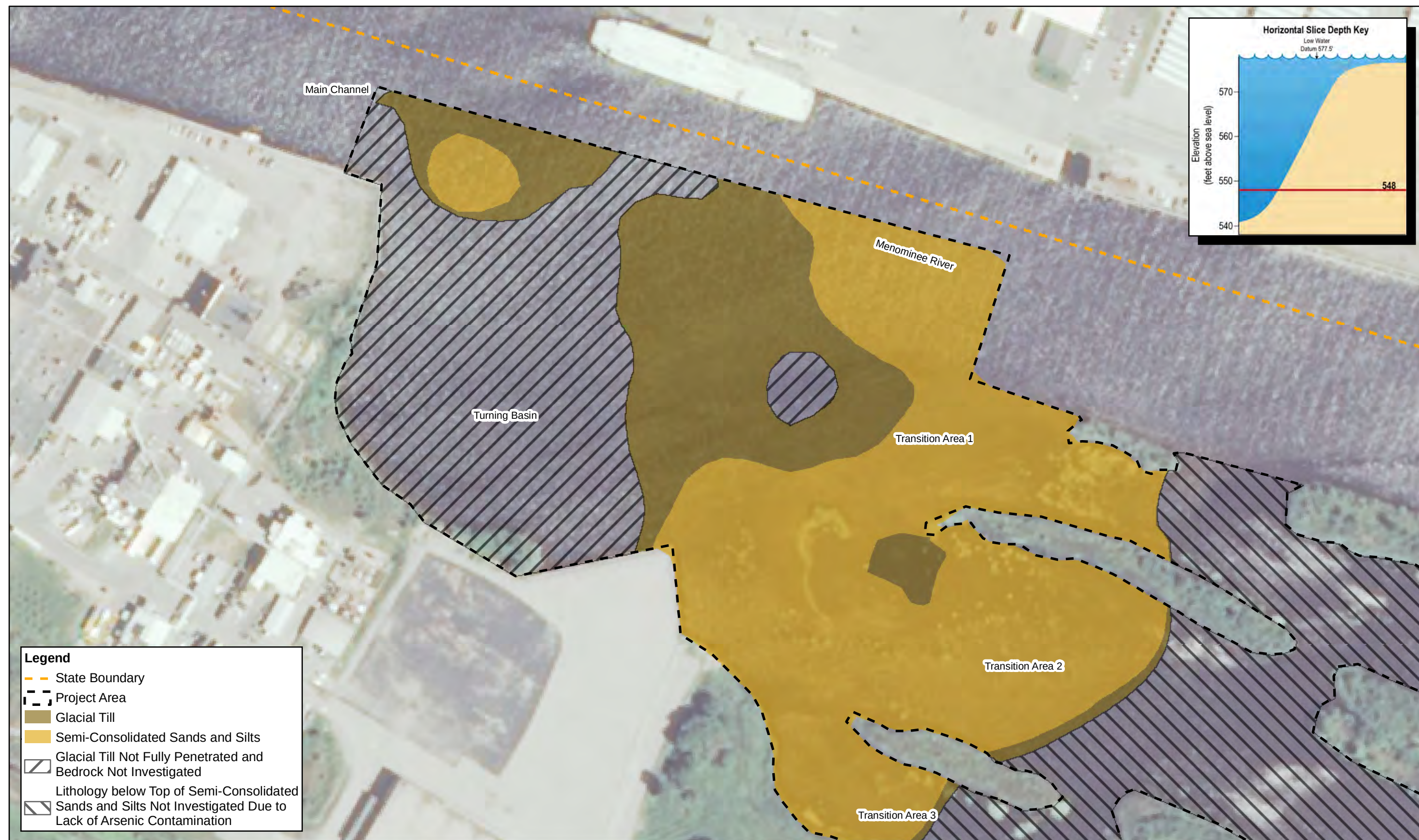
Figure 11B Horizontal Slice of Project Area Lithology Elevation 548' Tyco Fire Products LP Facility Marinette, WI
