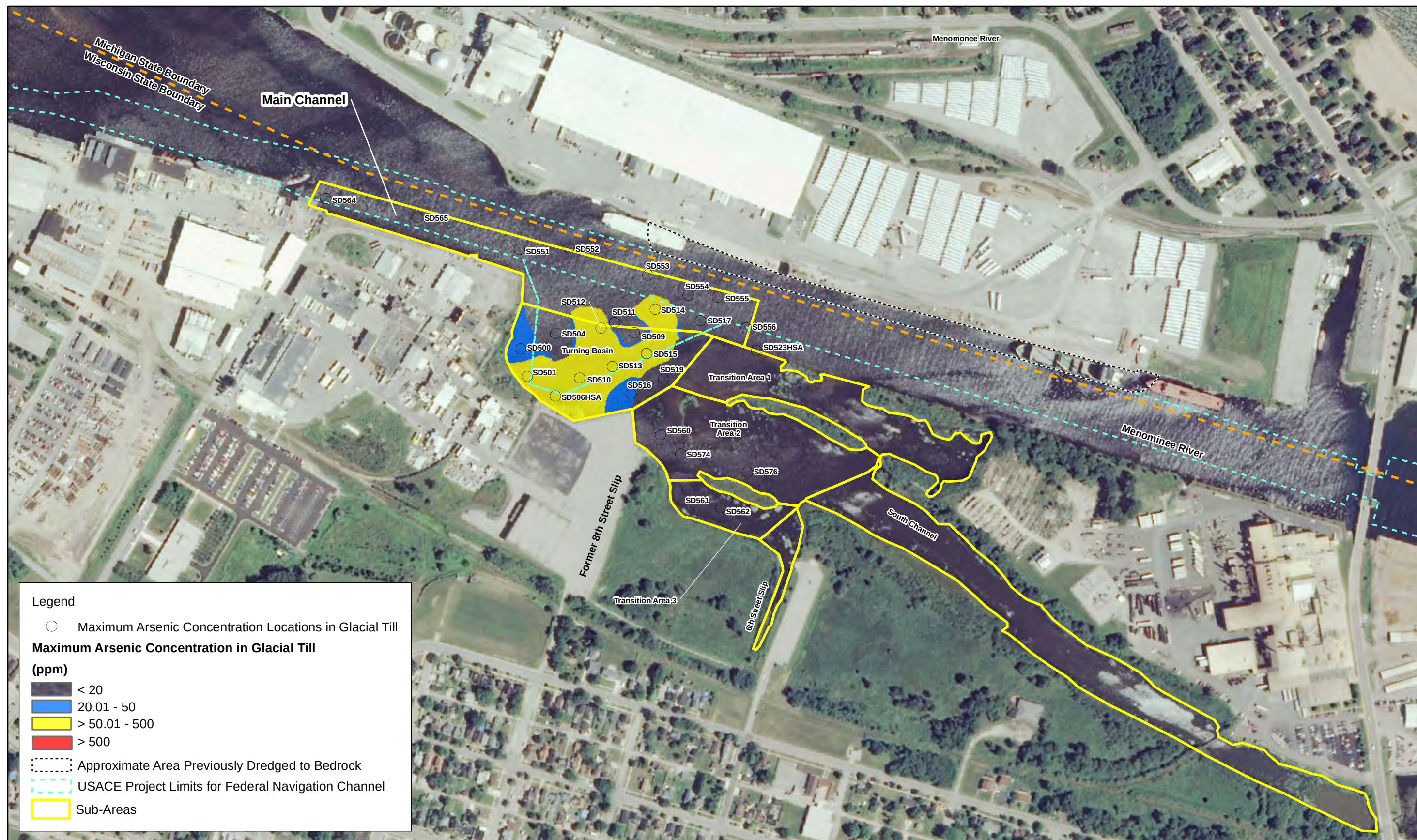
Figure 14 Maximum Arsenic Concentration in Glacial Till Tyco Fire Products LP Facility Marinette, WI
