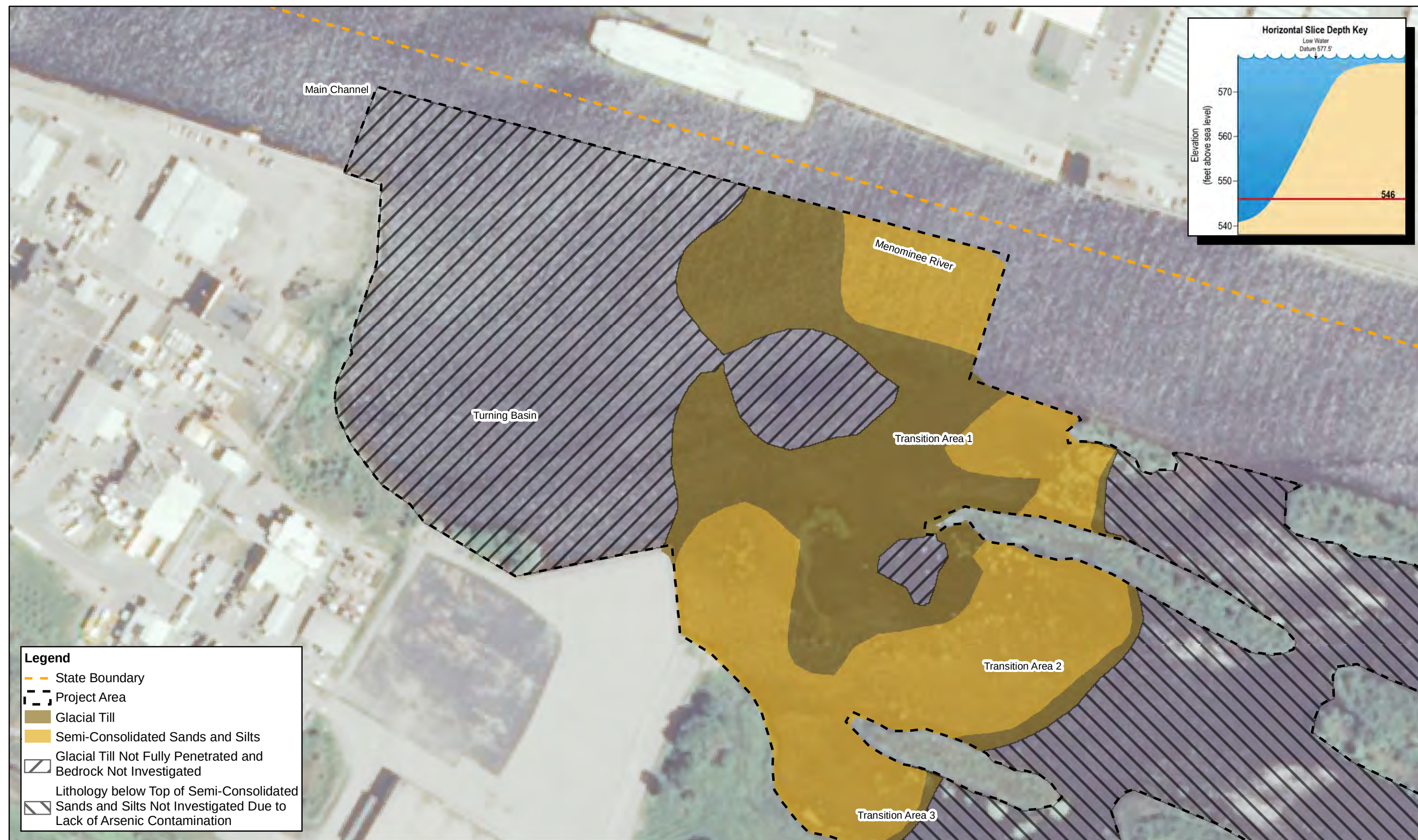
Figure 11A Horizontal Slice of Project Area Lithology Elevation 546' Tyco Fire Products LP Facility Marinette, WI
