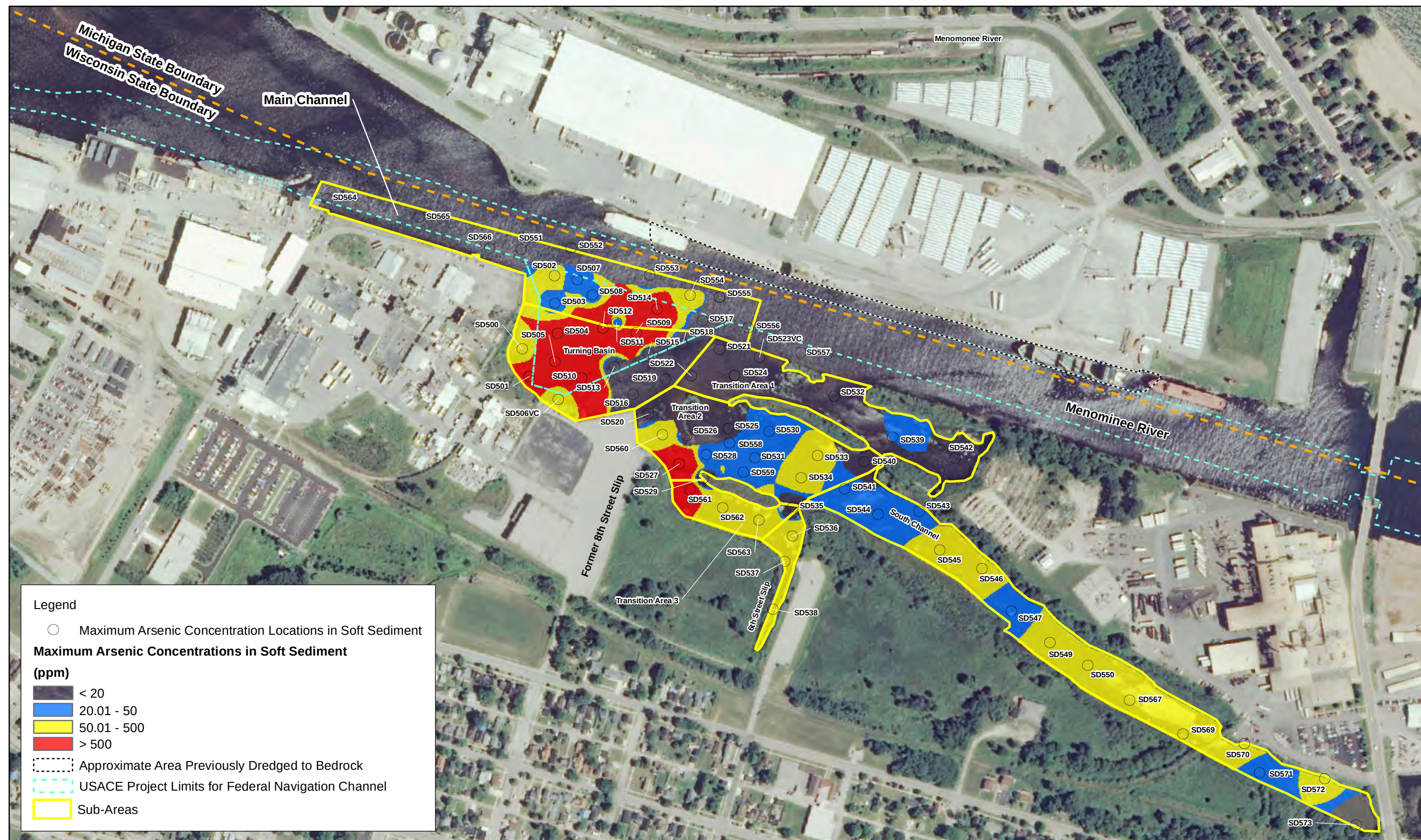
Figure 12 Maximum Arsenic Concentration in Soft Sediment Tyco Fire Products LP Facility Marinette, WI
