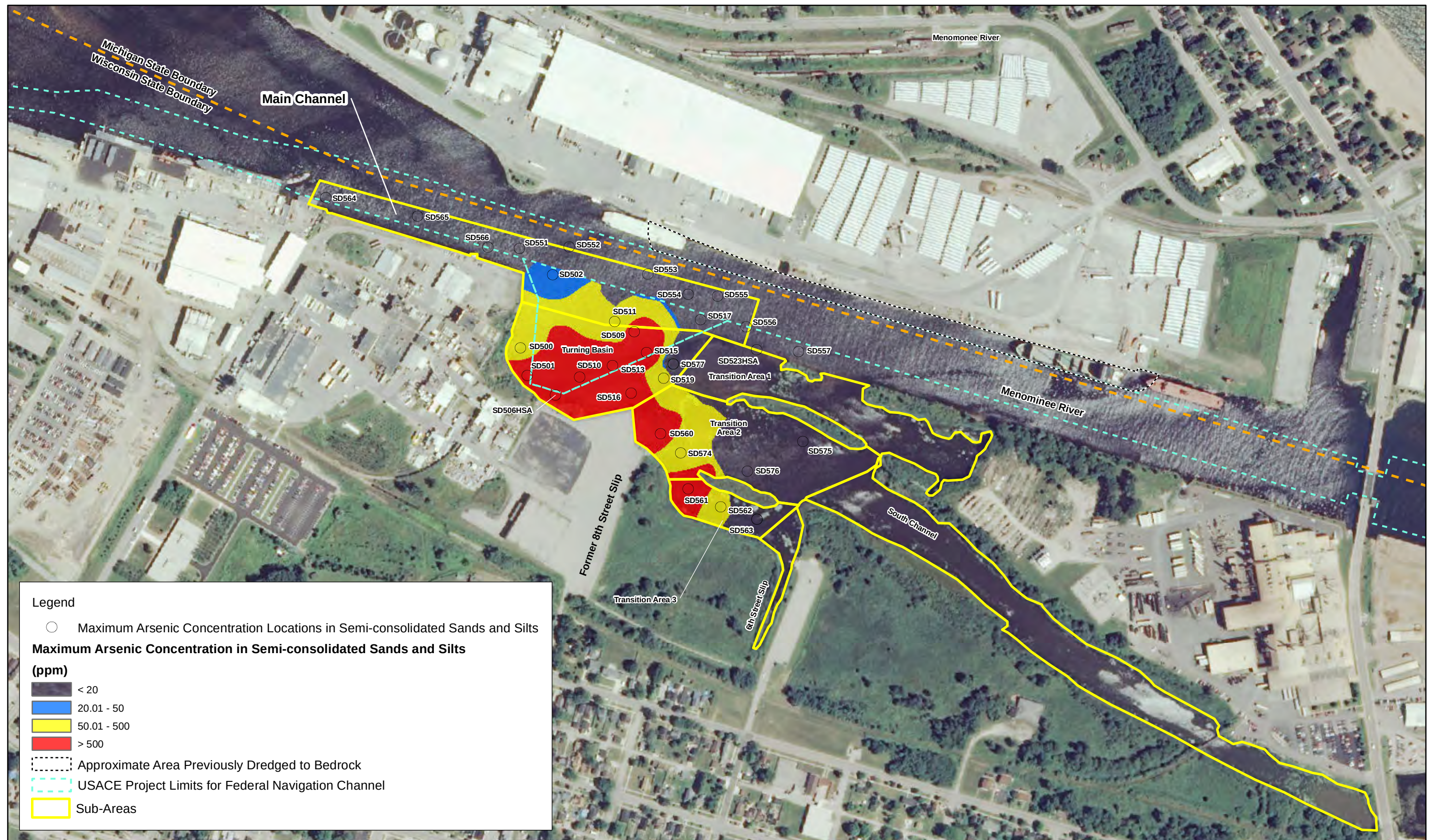
Figure 13 Maximum Arsenic Concentration in Semi-consolidated Sands and Silts Tyco Fire Products LP Facility Marinette, WI
