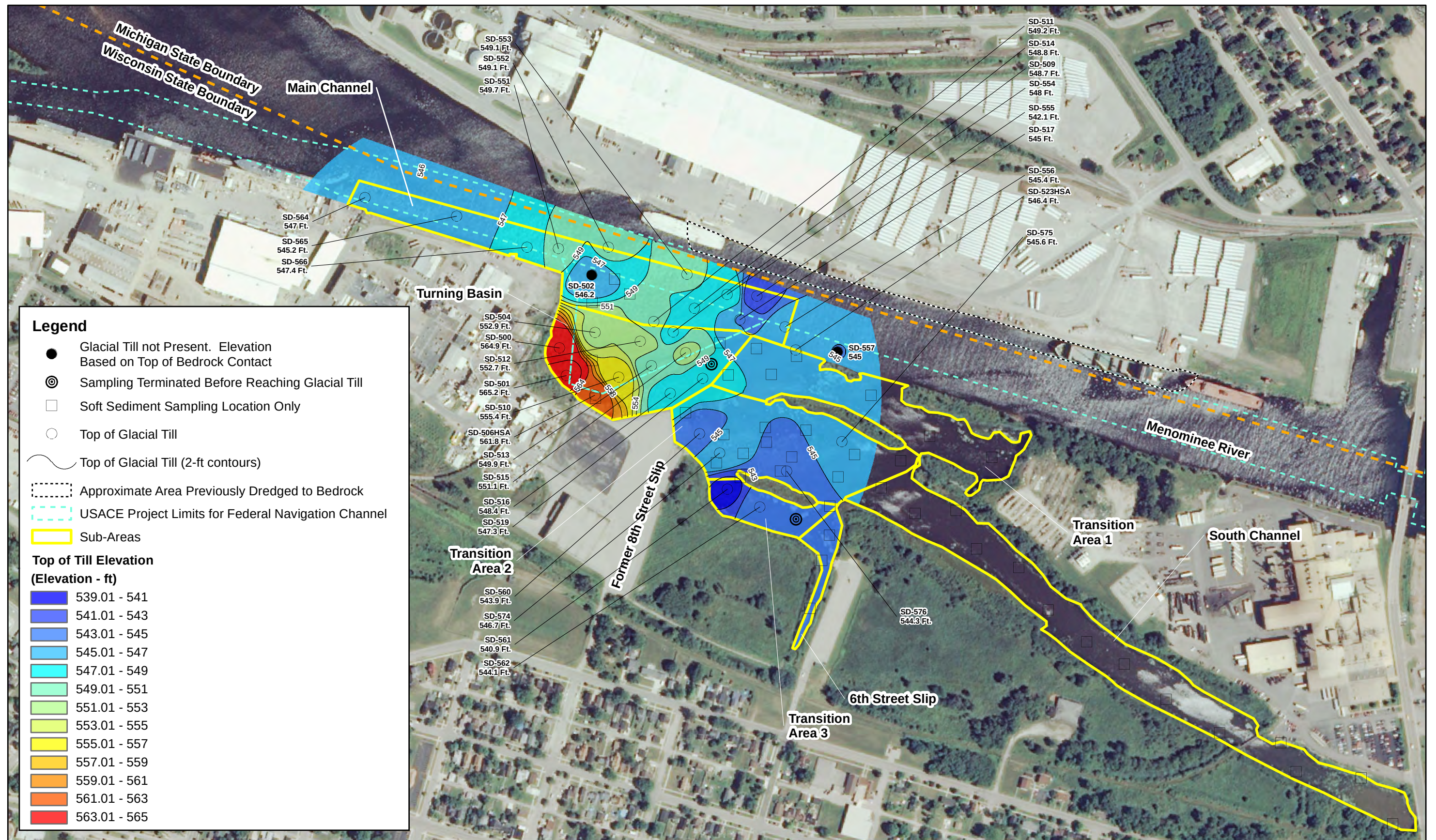
Figure 10 Top of Glacial Till Elevation Contours Tyco Fire Products LP Facility Marinette, WI
