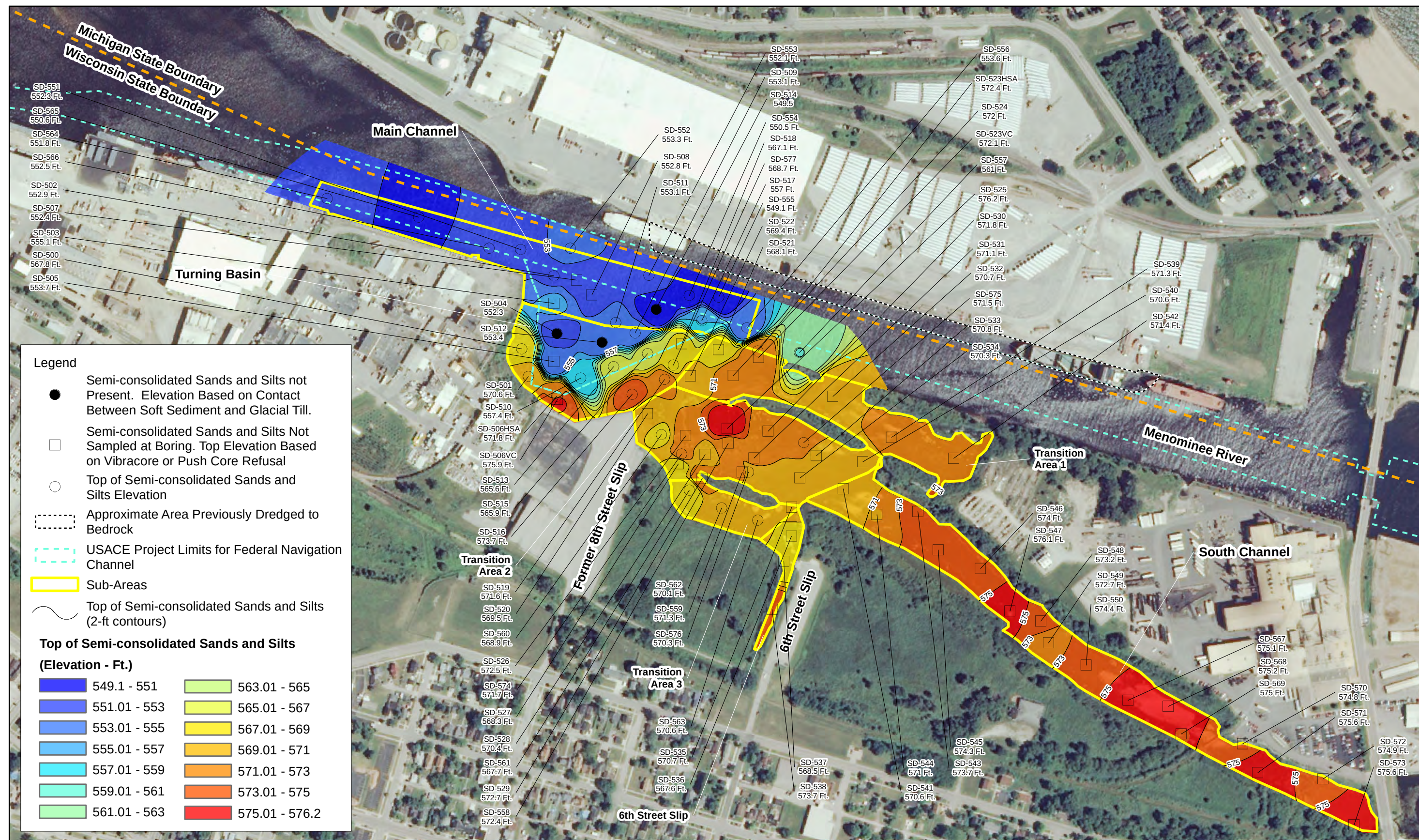
Figure 9 Top of Semi-consolidated Sands and Silts Elevation Contours Tyco Fire Products LP Facility Marinette, WI
