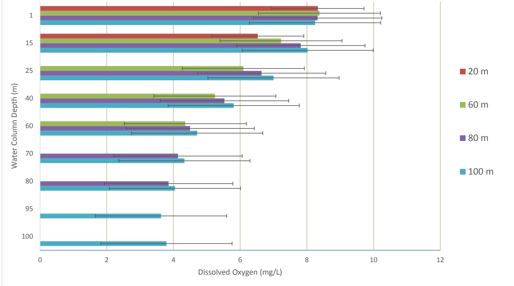
Figure A-6. Long-term average and standard deviation for Dissolved Oxygen at 20, 60, 80, and 100 meter contours (January 2008 through December 2013).
