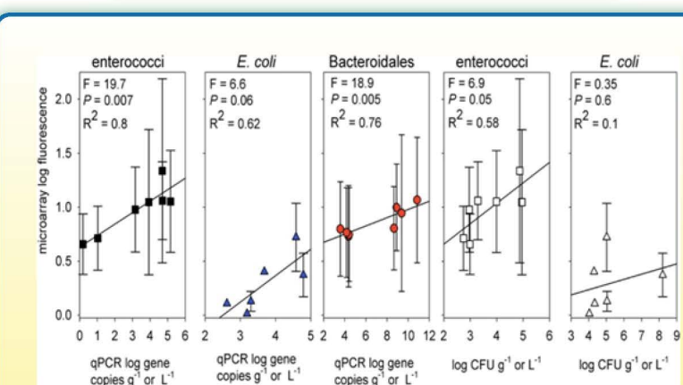
Figure 3. Correlation between microarray relative log fluorescence units (n = 6 perfect match probes) and microbial abundance determined via qPCR and culture methods. Average and standard deviation of microarray log fluorescence for multiple probes on the microarray targeting Enterococcus spp., E. coli , and Bacteroidales versus the qPCR log gene copies per L or g based on E. coli uidA gene, Bacteroidales (Genbac) 16S rRNA, and Enterococcus 23S rRNA.
