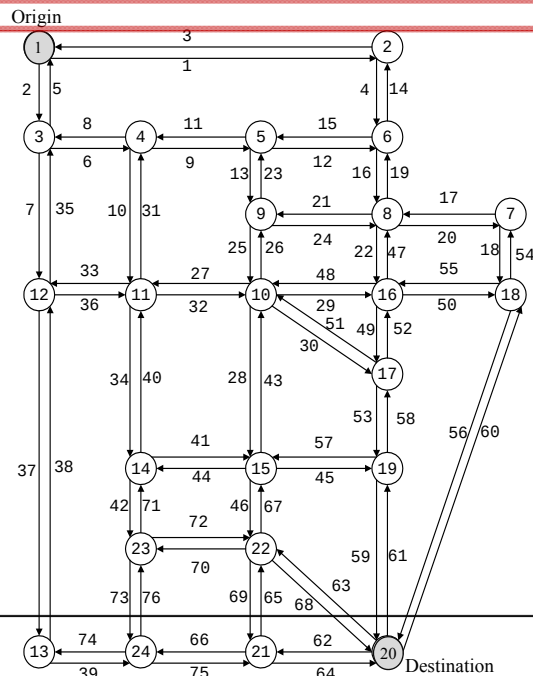
24-node and 76-link Sioux Falls network (Bar-Gera, 2009) nois.ed (Bar-Gera, 2009)
