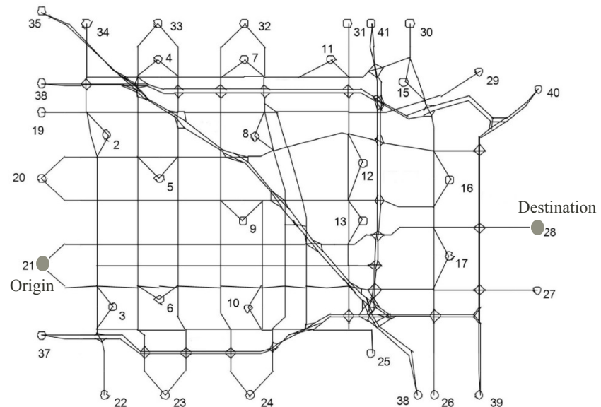
416-node and 914-link Anaheim network
