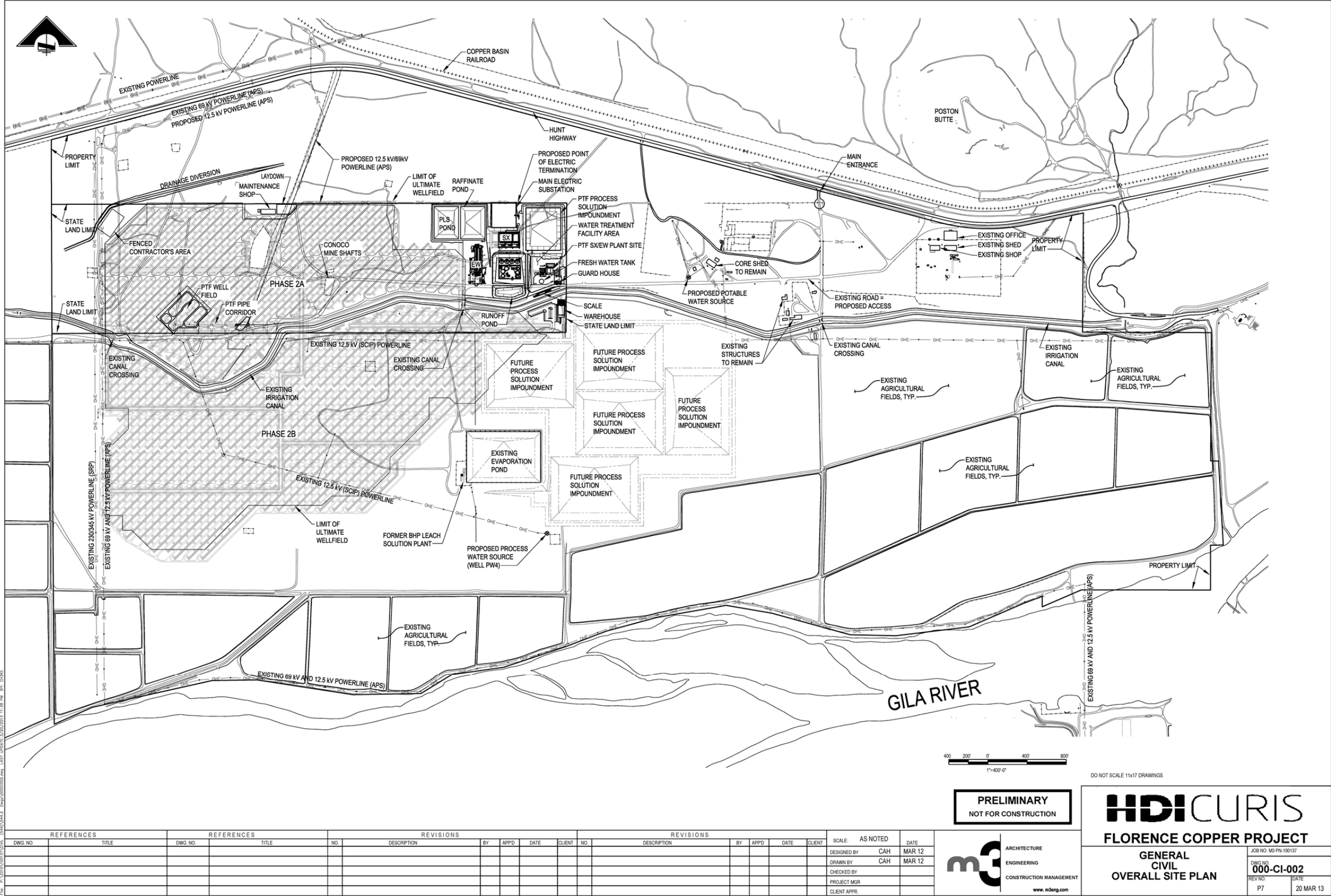
Figure 17-1: General Site Plan
