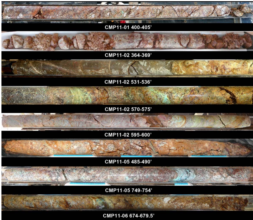
Figure 7-6: 2011 PQ Core- Bedrock Formations
