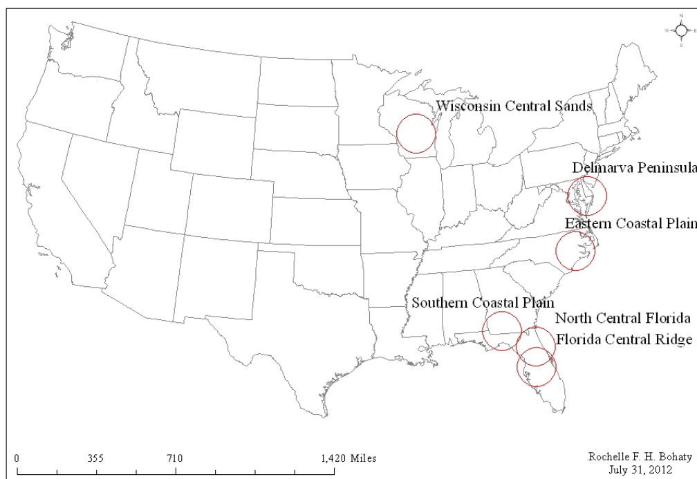
Figure 4.1. PRZM Groundwater Scenario Locations
