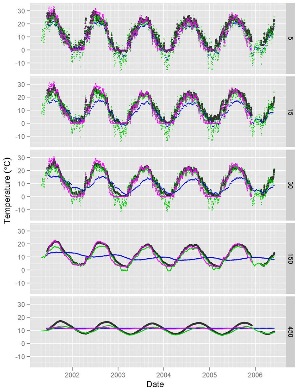
Figure 3.12. Temperature Simulation Comparison at the Study 5: Michigan Site for Depths of 5, 15, 30, 150, and 450 inches. The graph shows soil temperature measured at the weather station (black) as well as LEACHM (blue), PRZM (magenta), and PEARL (green) simulations
