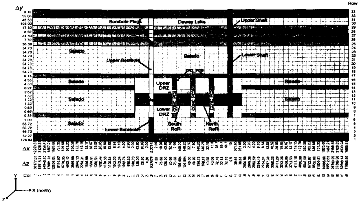
Figure 2-3: PABC-2009 BRAGFLO grid ( \Delta x , \Delta y , and \Delta z dimensions in meters).
