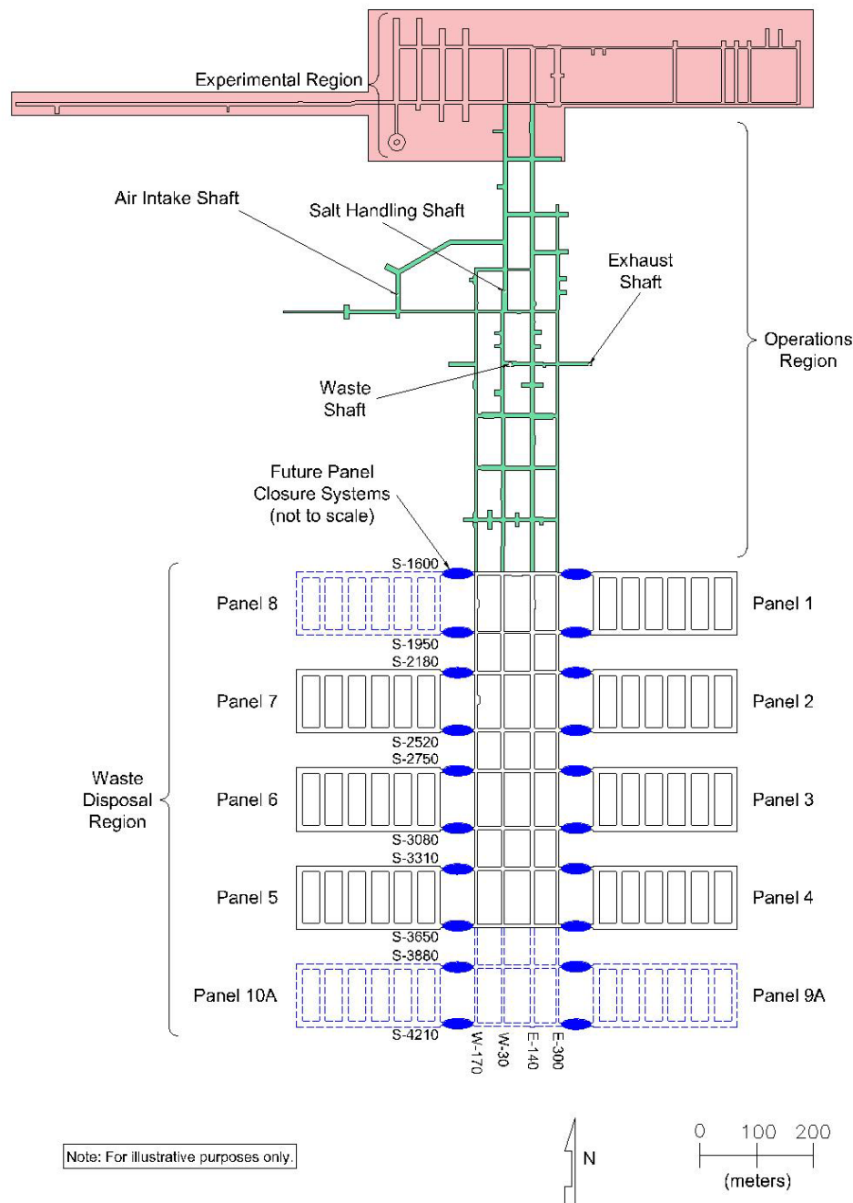
Figure 2. Plan view of the revised repository layout
