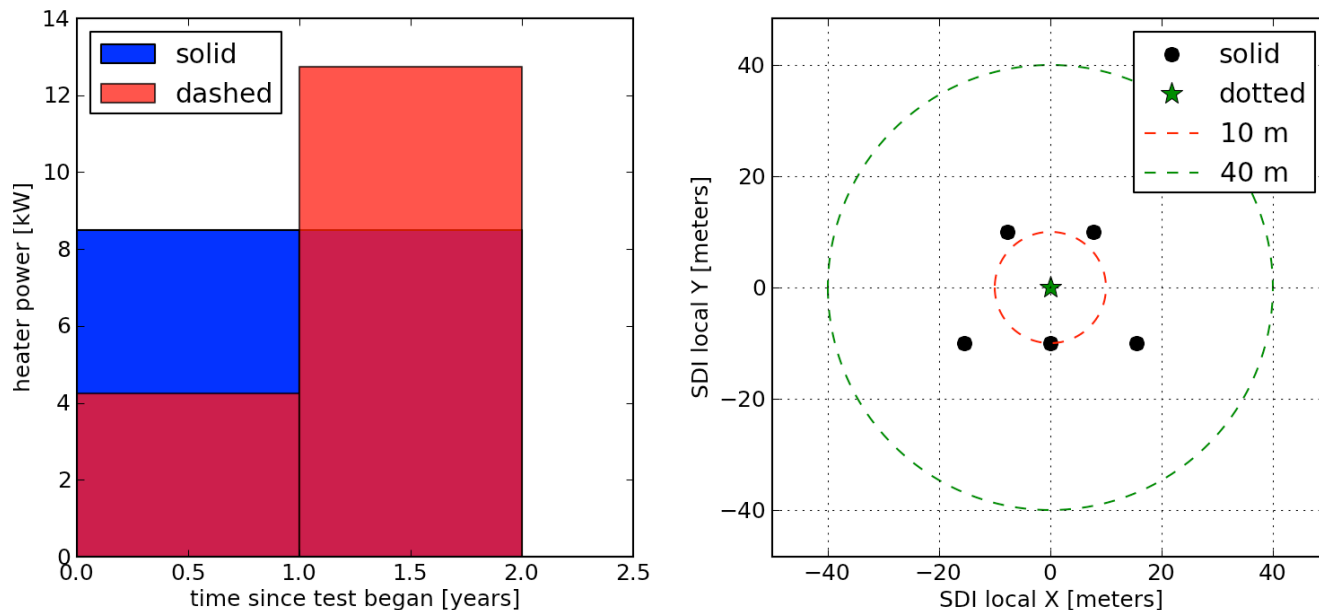
Figure 2. Illustrations of three different source-configuration scenarios in Figures 1 and 3. Left bar chart shows temporal variability in source between solid and dashed lines in Figures 1 and 3. Right map shows spatial locations of five proposed sources and single effective source in Figures 1 and 3. Dashed circles correspond to the two shortest distance curves plotted in Figure 1.
