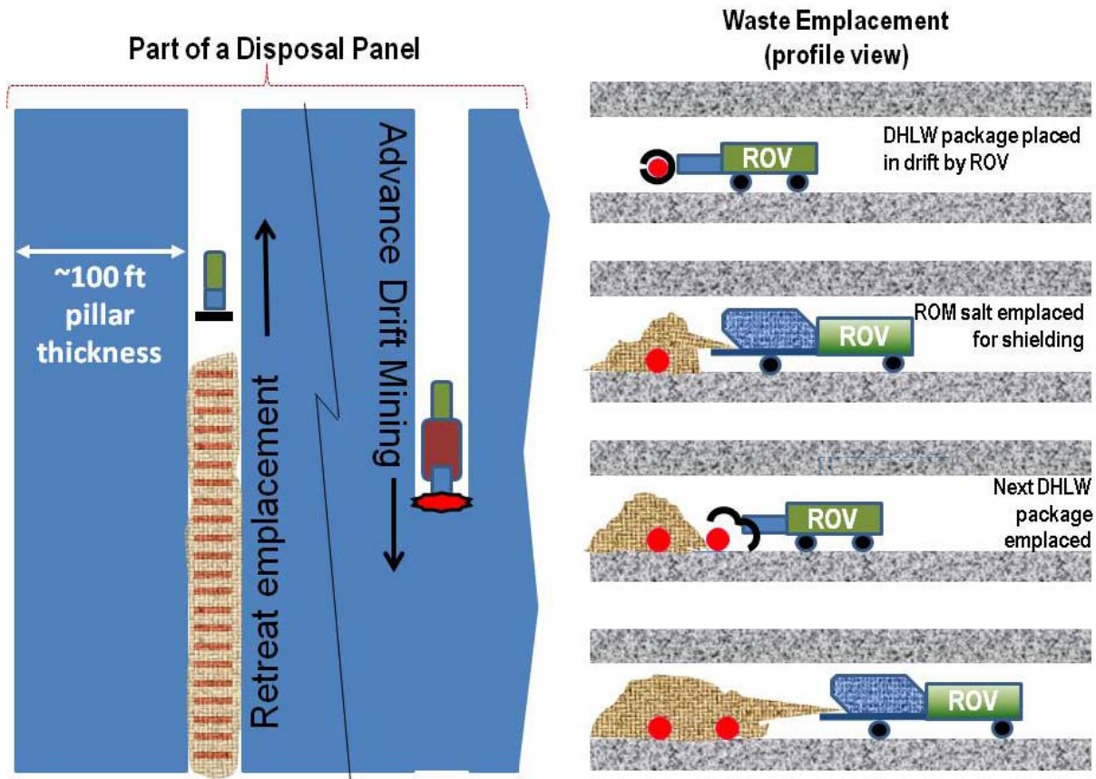
Figure 2-1: In-Drift Waste Emplacement Concept
