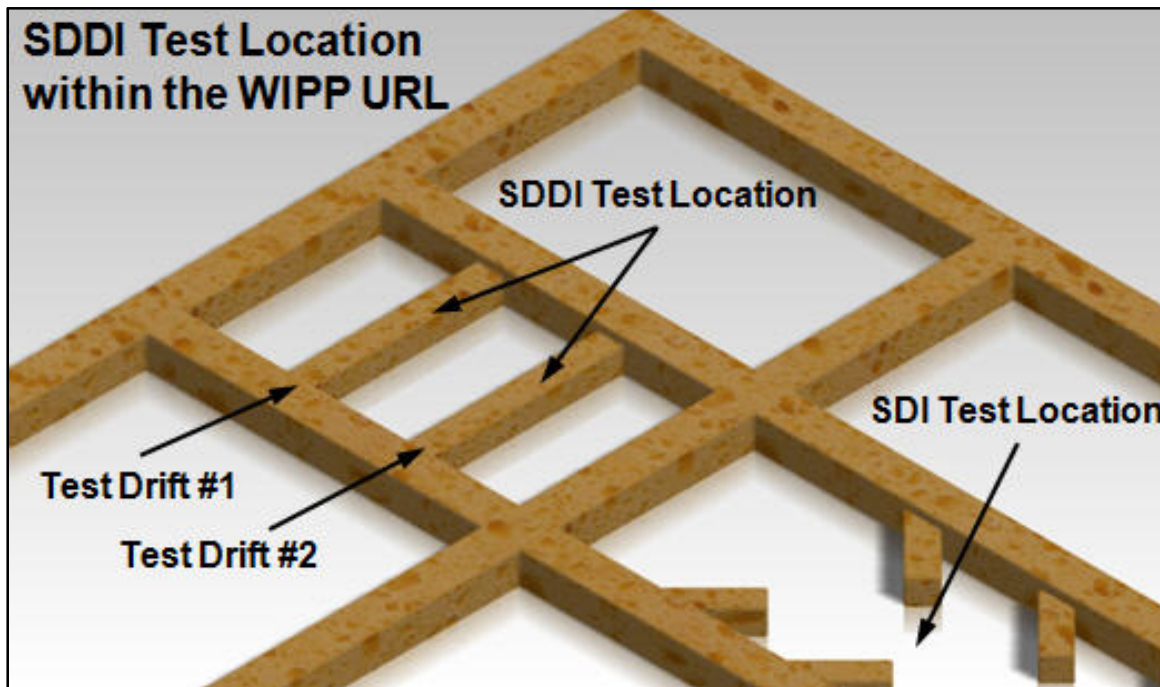
Figure 3-3: Perspective View of the Mining Layout for the SDDI Thermal Test
