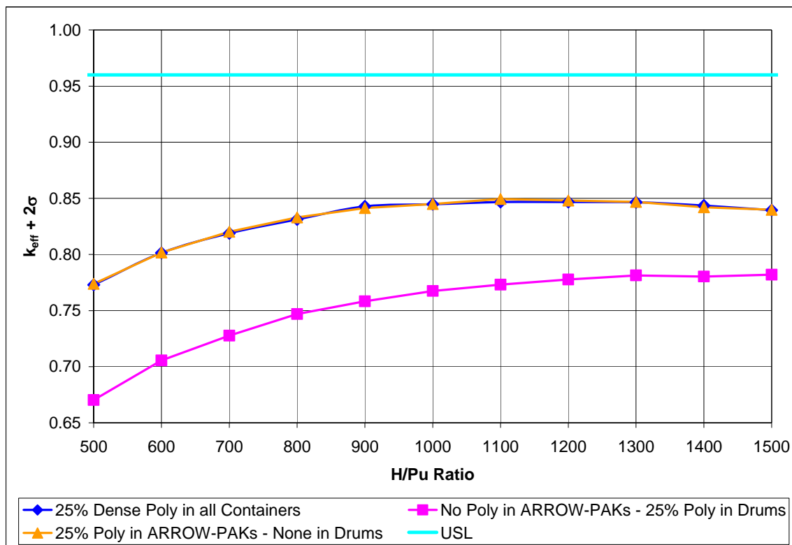
Figure A-, Underground Array Reactivity for ARROW-PAK™ Containers with Seven-pack of 55-gallon Drums on Top
