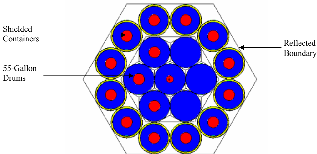
Figure -, Drum Array with Shielded Containers, X-Y Plane
