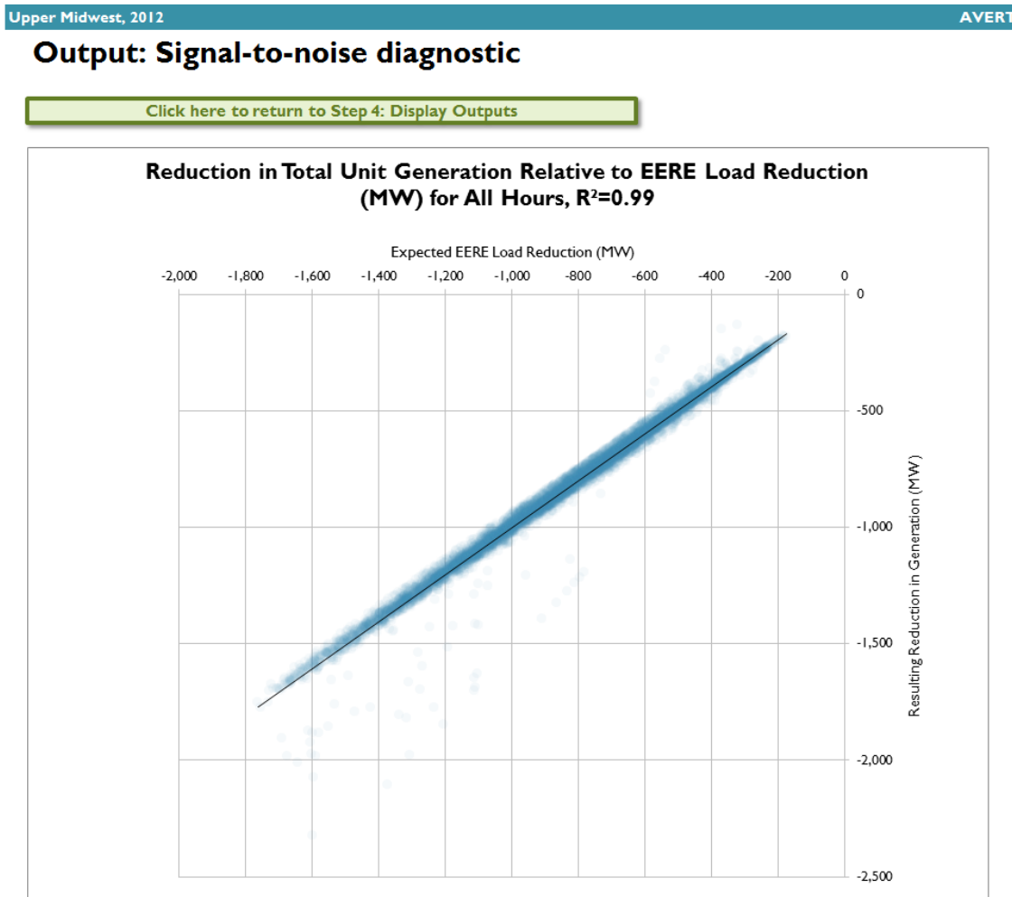
Figure 24. Signal-to-noise diagnostic for an example wind program in the Upper Midwest region.
