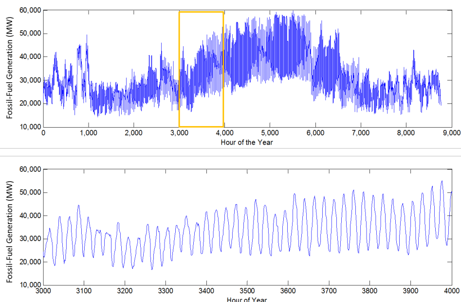
Figure 27. 2011 hourly sum of fossil-fuel generation in the Texas region.
