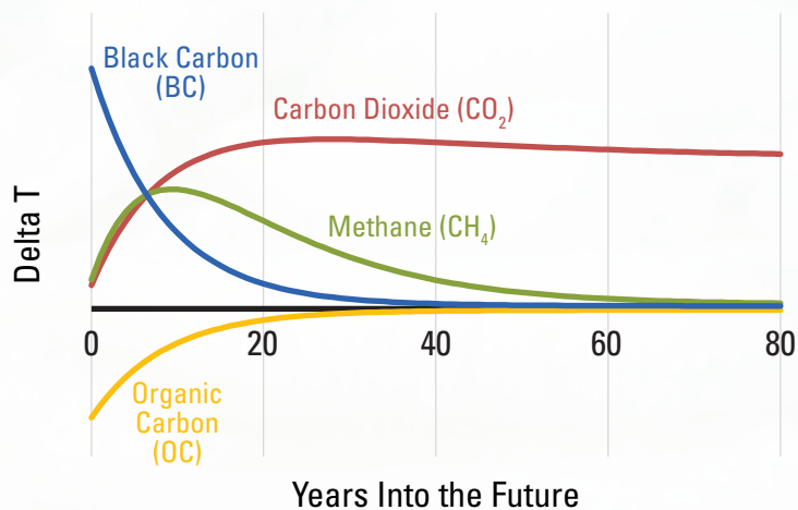
Figure 4. Temperature responses by pollutant for total anthropogenic emissions for one-year emissions pulses. Derived from: IPCC, 2014.
