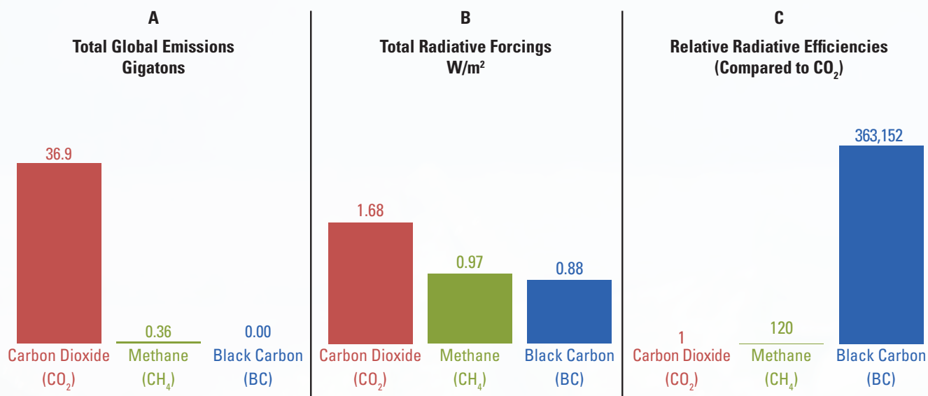
Figure 3. Comparison of carbon dioxide, methane, and black carbon's total global emissions (A), total radiative forcings (B), and relative radiative efficiencies (C). Sources: Bond et al., 2013; IPCC, 2014.
