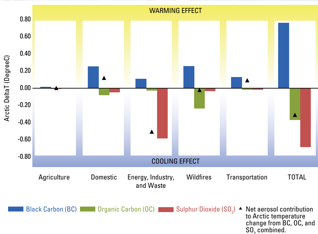
Figure 6. Arctic temperature change resulting from 2010 emissions of black carbon and co-emitted pollutants by sector. Derived from: Wobus et al., 2016.
