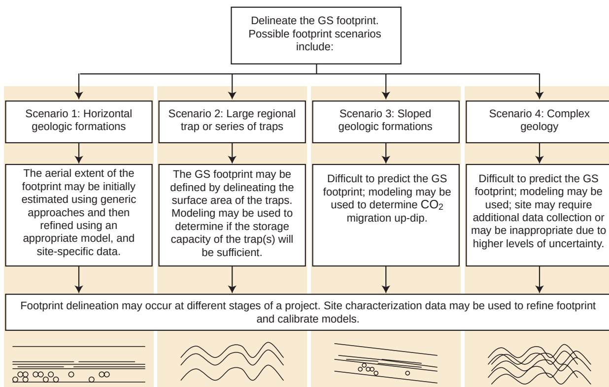
Figure 3.5. Geologic Sequestration (GS) Footprint Delineation
