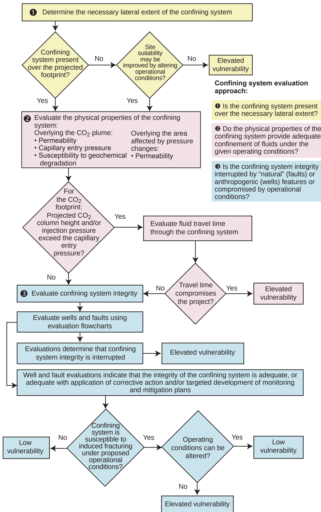
Figure 3.2. Confining System Evaluation
