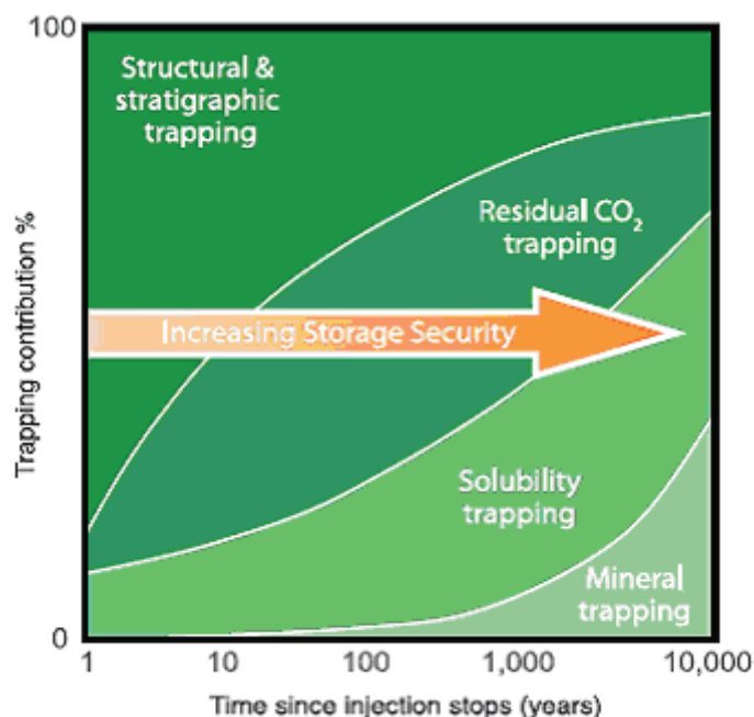
Figure 2.2. Effectiveness of Trapping Mechanisms Over Time. Source: IPCC, 2005, Figure 5.9.
