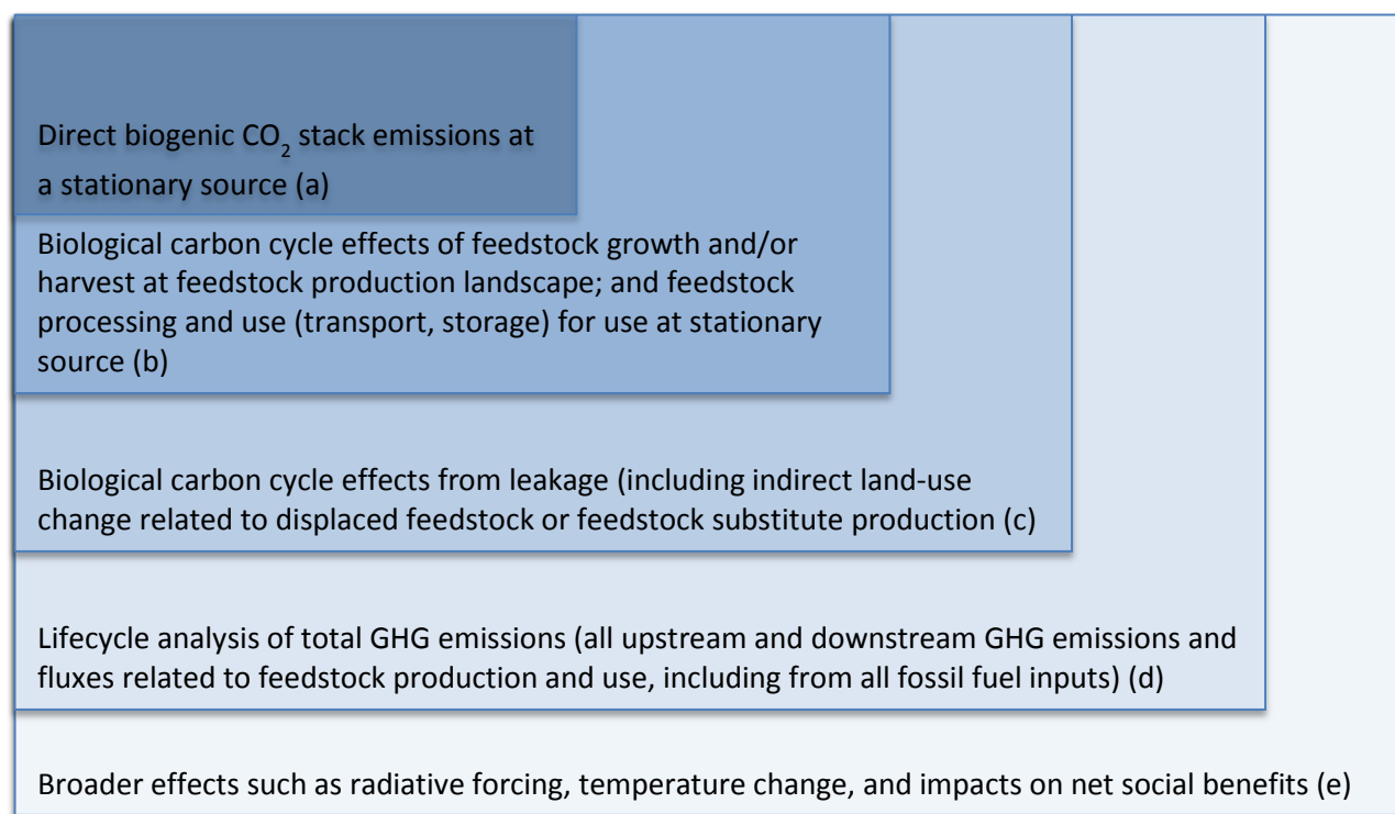
Figure 3: Potential Range of Assessment Scope. The framework focuses on the first three boxes (a through c). Though an equation term for leakage is included in the framework equation, a method for calculating leakage is not provided in this report. This framework does not include a complete lifecycle GHG emissions analysis (d) or include analysis of temperature change impacts, radiative forcing, and impacts on net social benefits (e).
