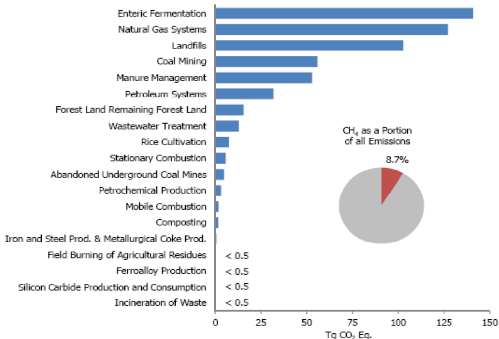
Figure 4: The Relative Size of Methane Emission Sources in the U.S. in 2012 (EPA, 2014).
