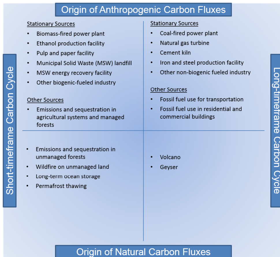
Figure 2: Various Carbon Flux Types and Time Frames. Carbon fluxes with the atmosphere can be defined in terms of (1) the long-term carbon cycle common to fossil fuels versus the short-term carbon cycle common to biogenic feedstocks and (2) natural versus anthropogenic origin of emissions.
