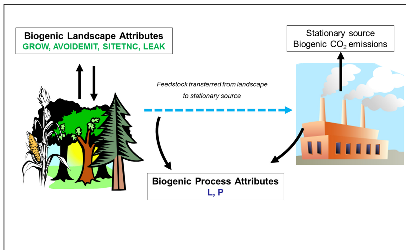
Figure 5: Diagram with Equation Terms Included. This figure is the same as Figure 4 except that in addition to illustrating the basic processes (i.e., biogenic carbon and carbon fluxes) addressed in the framework, this graphic also includes the equation terms that represent each of these basic process elements. The framework addresses biogenic carbon flows and fluxes associated with the production, processing, and use of a biogenic feedstock, including biogenic carbon impacts at the production landscape ( GROW, AVOIDEMIT, SITETNC ) as well as indirect impacts on landscapes other than the production landscape ( LEAK ); biogenic feedstock carbon losses during transport, storage, and processing of the feedstock ( L ); and biogenic feedstock carbon that is embodied in products that exit the supply chain or stationary source in means other than the stack ( P ).
