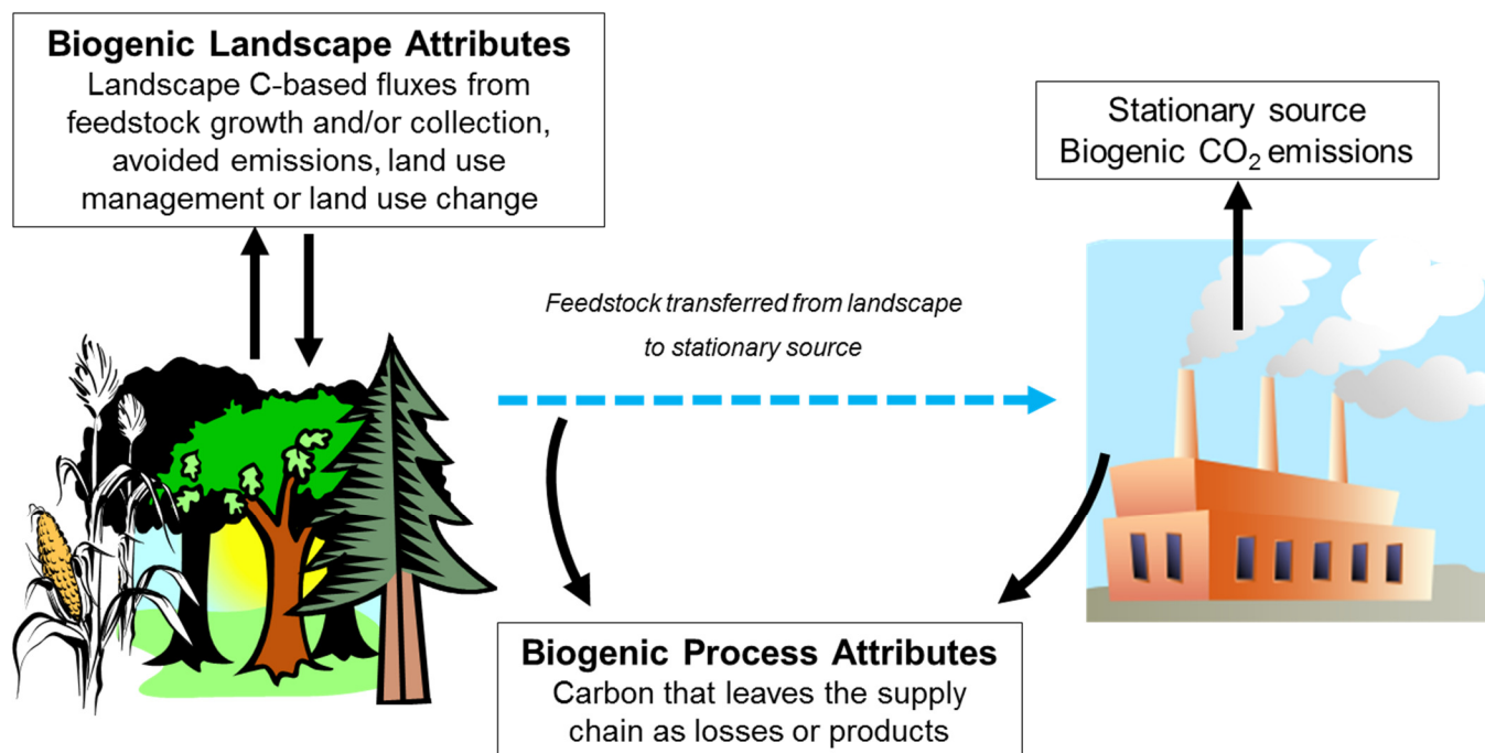
Figure 1. Diagram Illustrating the Basic Processes Addressed in the Framework. The framework addresses carbon fluxes associated with production, processing, and use of biogenic feedstocks. The solid, black arrows represent flows of carbon to and from the system of feedstock growth, harvest, and use. The dashed, blue arrow represents physical transfers of the biogenic feedstock from the production landscape to the stationary source (transport-related emissions such as tractor or train fuel are not included in the framework).
