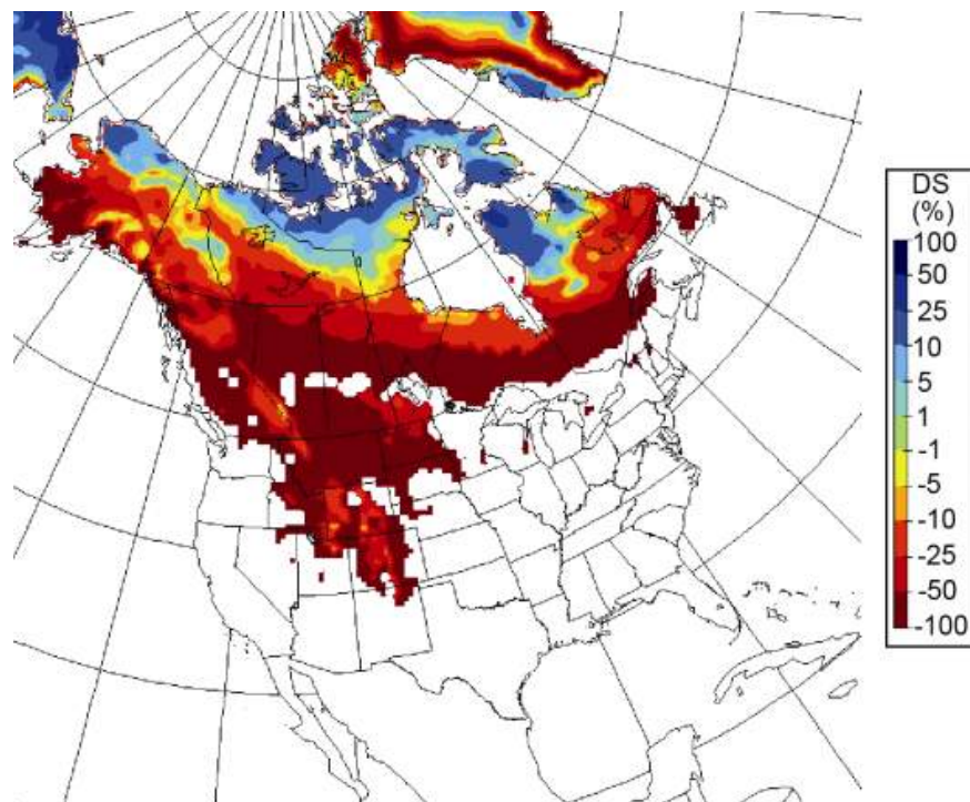
Figure 6.10: Percent Snow Depth Changes in March
