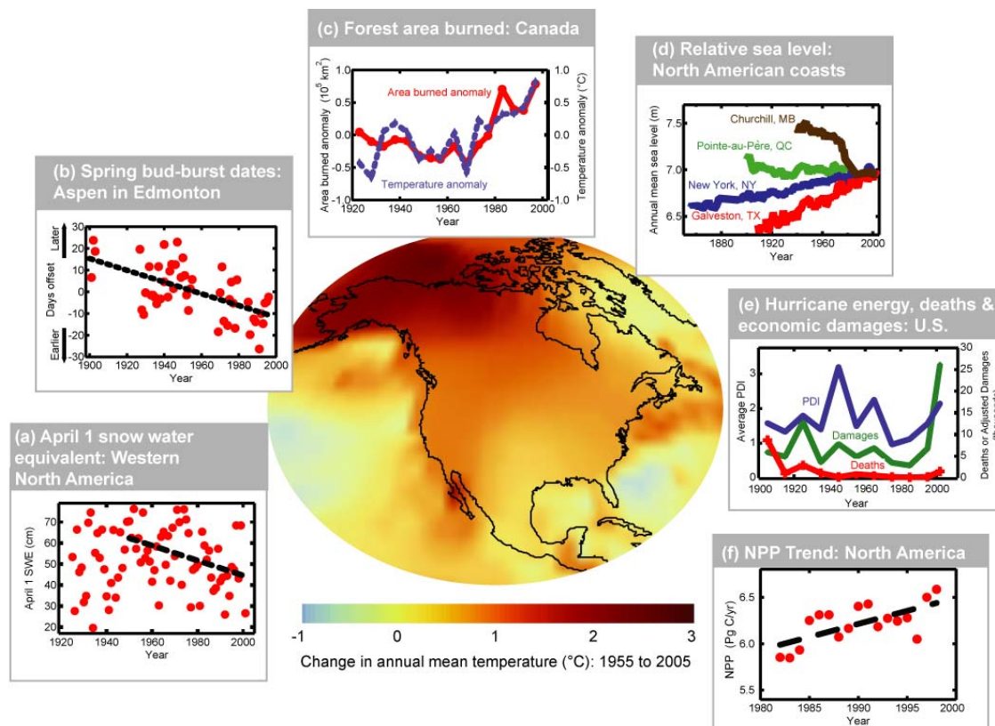
Figure 14.1: North American Observations
