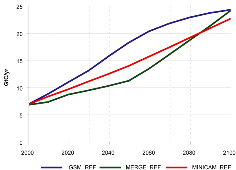
Figure 6.2: Projected Global Emissions of CO 2 from Fossil Fuels and Industrial Sources Across CCSP Reference Scenarios
