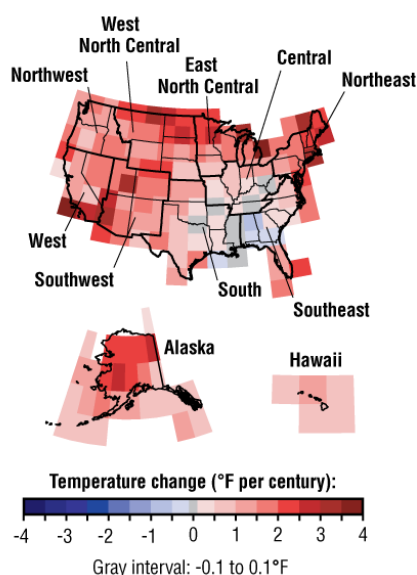
Figure 4.4: Map of the United States, Depicting Regional U.S. Temperature Trends for the Period 1901 to 2008 32
