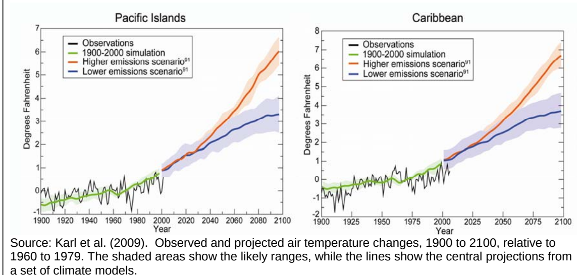
Figure 15.5: Pacific and Caribbean Island Air Temperature Change
