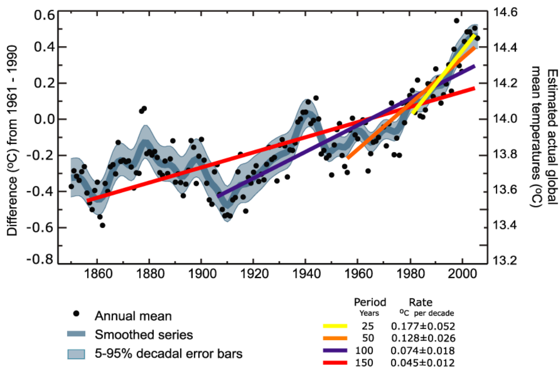
Figure 4.2: Annual Global Mean Temperatures (black dots) with Linear Fits to the Data.
