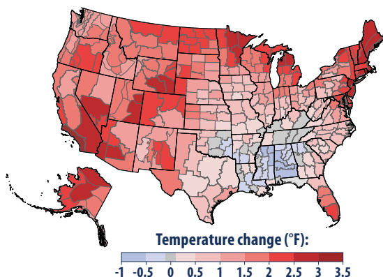
Rising temperatures in the last century. The warming in Oregon has been similar to the average warming nationwide. Source: EPA, Climate Change Indicators in the United States.
