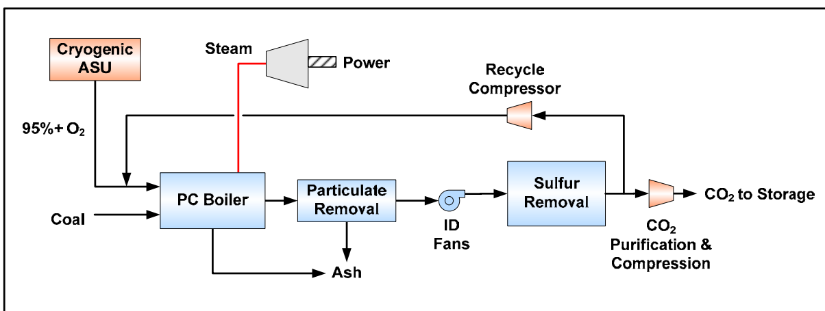
Figure A-6. Pulverized Coal Power Plant with Oxy-Combustion CO 2 Capture
