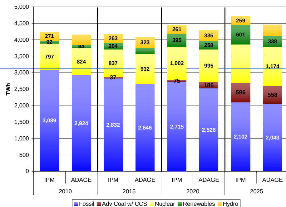
S. 2191 Scenario Electricity Generation Mix
