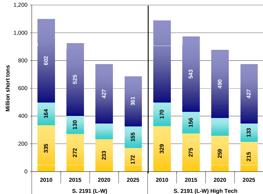
Coal Production for Electricity Generation
