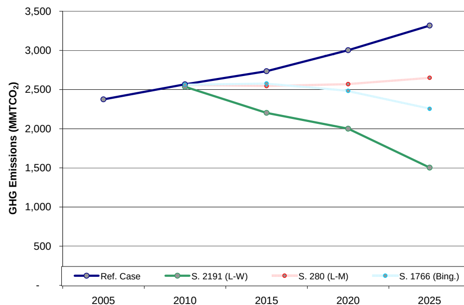
Power Sector CO 2 Emissions
