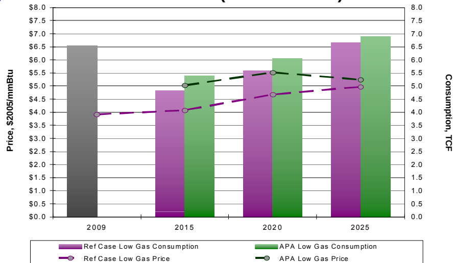
Natural Gas Consumption and Average N. Gas Delivered Prices (Electric Power)
