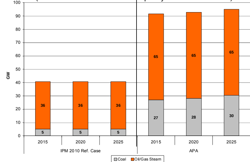
Retirements of Existing Capacity, Cumulative (Total Coal + Oil/Gas Steam capacity is around 430 GW)
