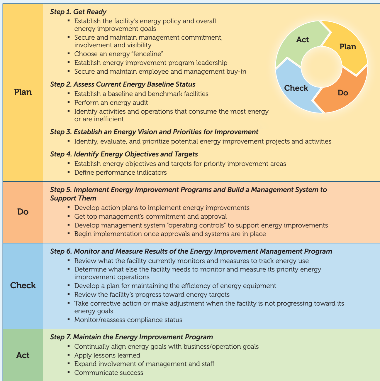
FIGURE 2. STEPS FOR DESIGNING, IMPLEMENTING, AND SUSTAINING ENERGY EFFICIENCY IMPROVEMENTS IN WATER AND WASTEWATER FACILITIES
