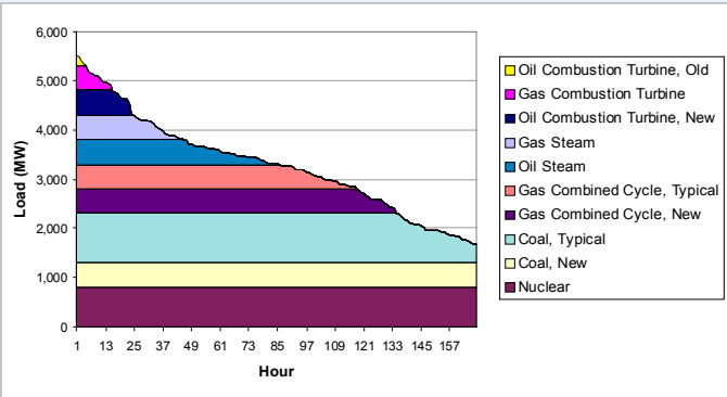
FIGURE 3.2.3 A HYPOTHETICAL LOAD DURATION/DISPATCH CURVE REPRESENTING 168 HOURS (shown in half-day increments) by generation unit, ranked by load level
