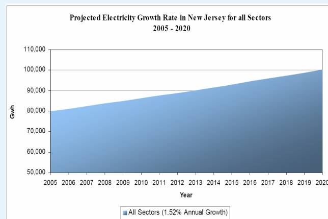
FIGURE 2.2.6 NEW JERSEY ENERGY PLAN-BASIC DEMAND FORECAST
