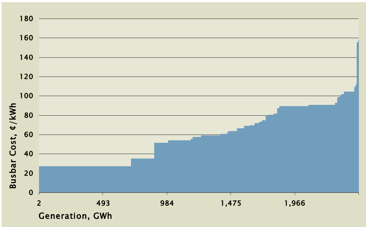
Figure D-9. Levelized Cost Supply Curve for Low Impact Hydro Generation.
