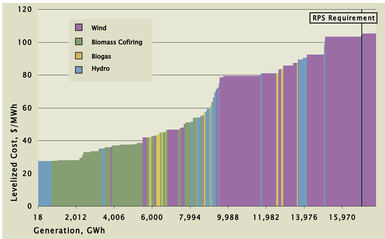
Figure A-1. Near-Term Potential Renewable Energy Generation Supply Curve.
