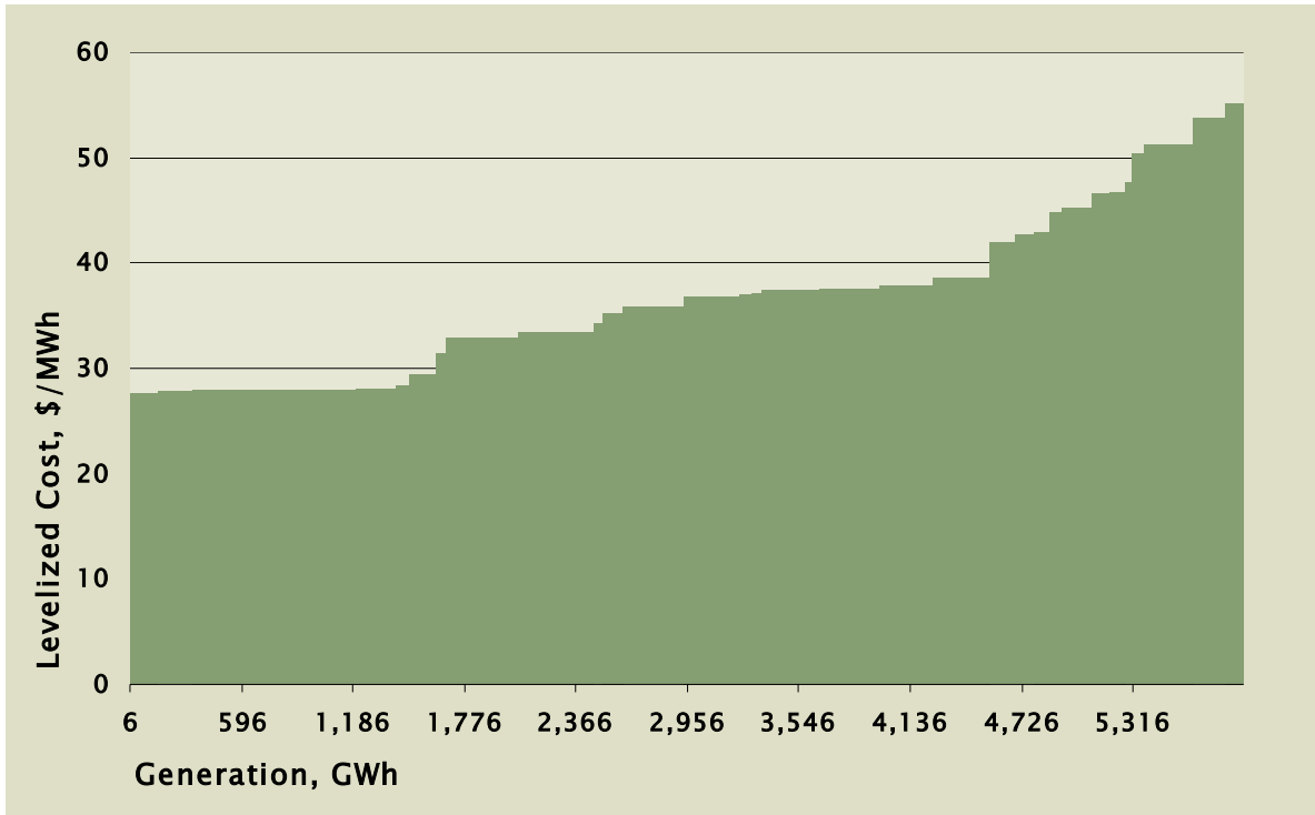
Figure D-5. Levelized Cost Supply Curve for Biomass Cofiring.
