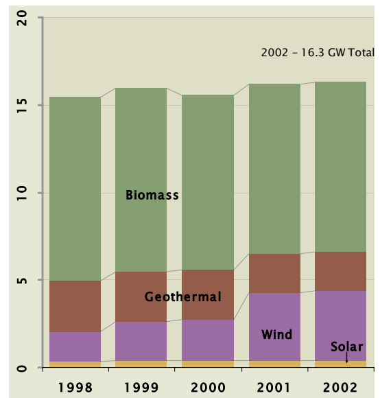
Figure B-2. US Net Renewable Electrical Capacity, GW. (EIA 2002)
