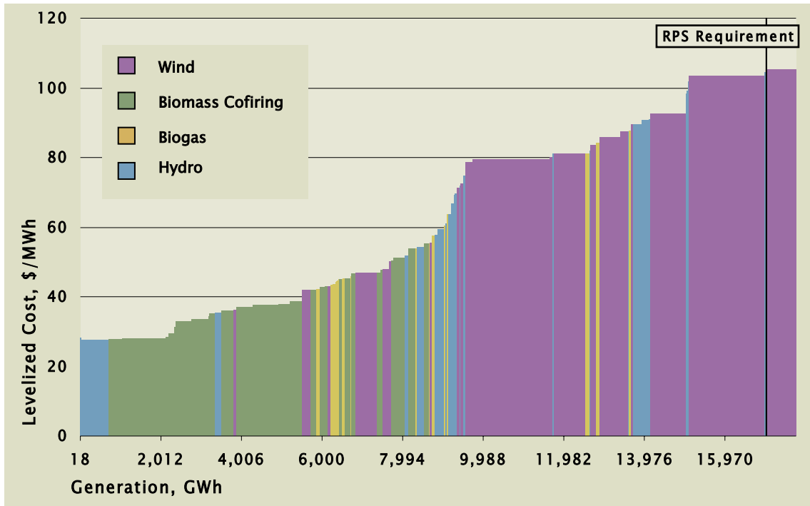
Figure D-1. Near-Term Potential Renewable Energy Generation Supply Curve.
