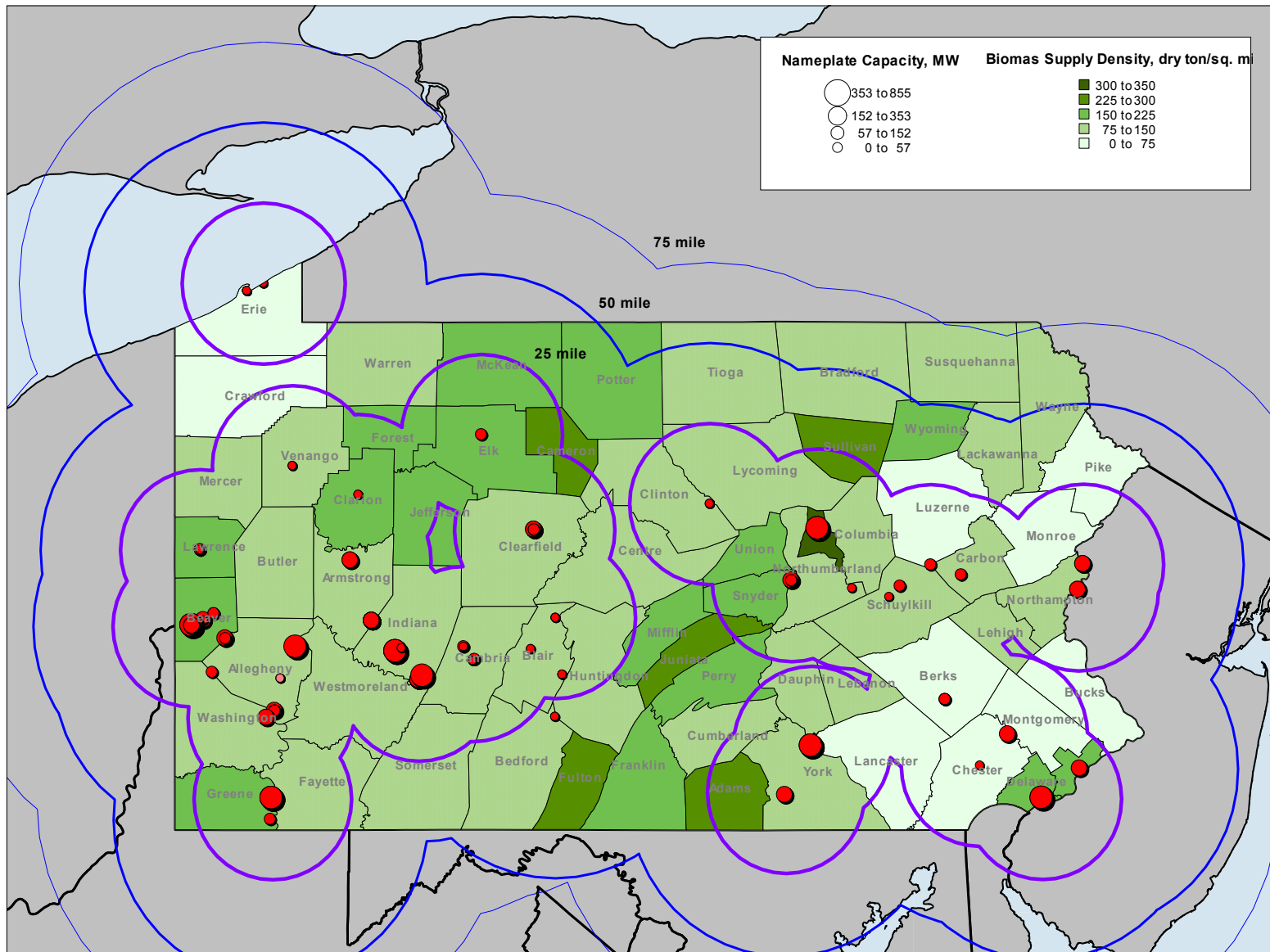
Figure D-4. Map of Installed Coal-Fired Generation and Biomass Resource Distribution.
