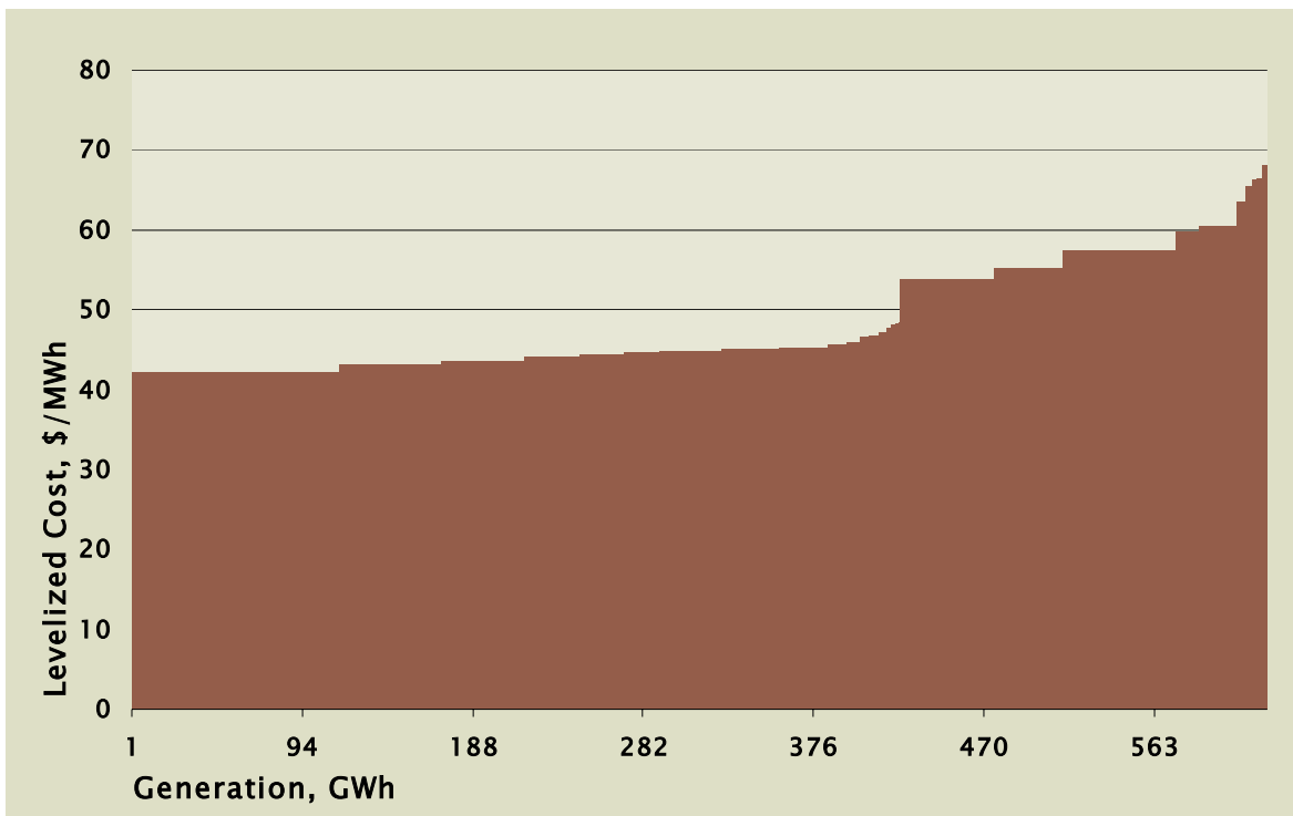
Figure D-6. Levelized Cost Supply Curve for Landfill Gas Power Generation.
