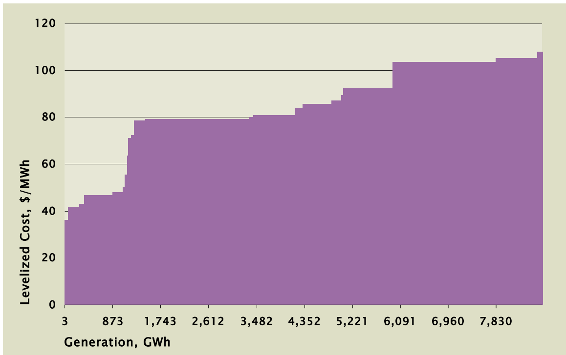
Figure D-2. Levelized Cost Supply Curve for Wind Energy.
