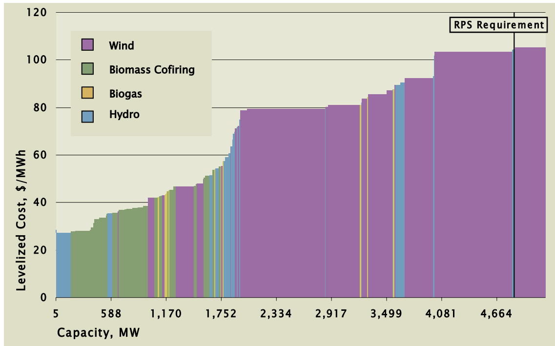
Figure D-11. Near-Term Potential Renewable Energy Capacity Supply Curve.
