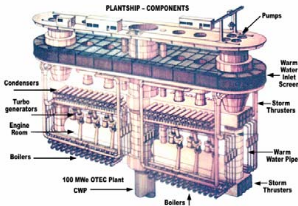
Figure 5-12. OTEC Schematic Diagram. (Source: www.seasolarpower.com )
