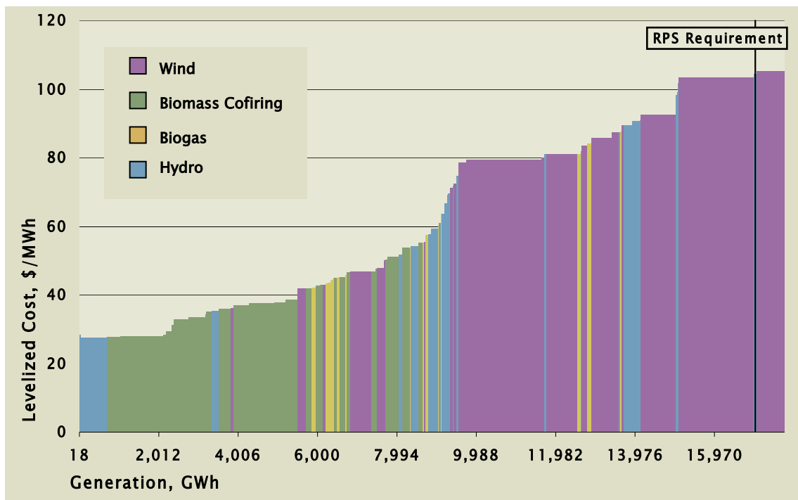
Figure D-10. Near-Term Potential Renewable Energy Generation Supply Curve.
