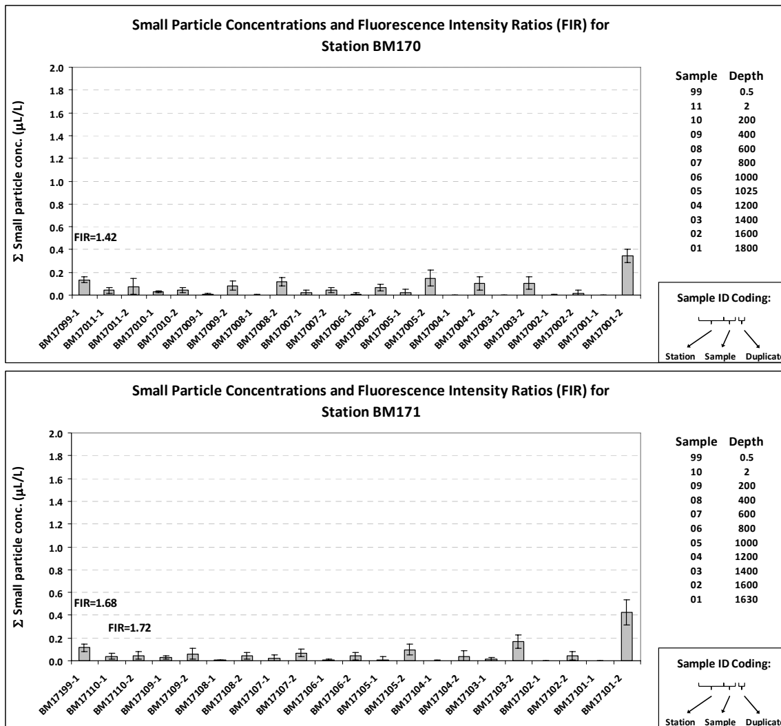
Figure 1: Average small particle concentrations and fluorescence intensity ratios as a function of depth for stations BM169 to BM171.
