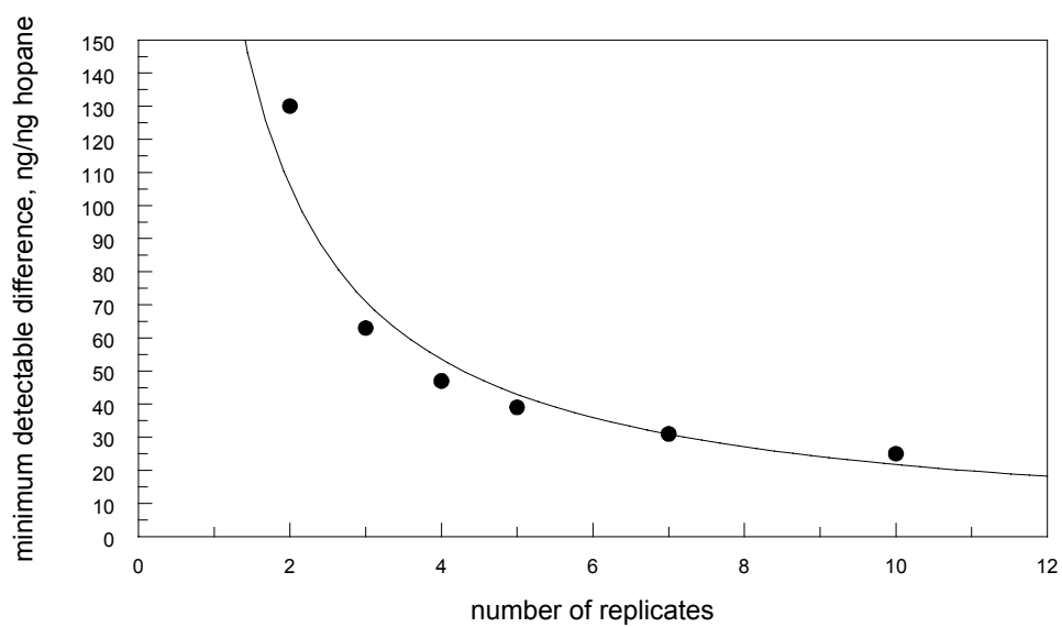
Figure 6.3. Minimum detectable treatment difference as a function of number of replicate plots.
