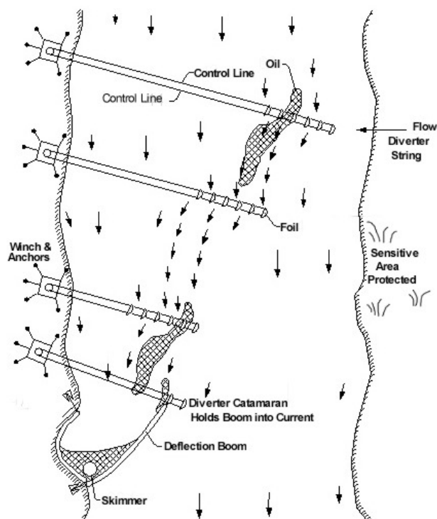
Figure 1. Flow Diverters in a Cascade Tactic
