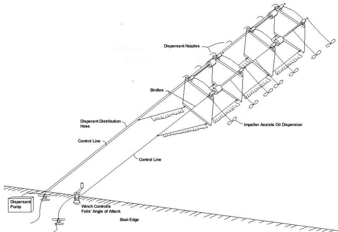
Figure 13. Oil Dispersant Deployed and Mixed by the Diverter System
