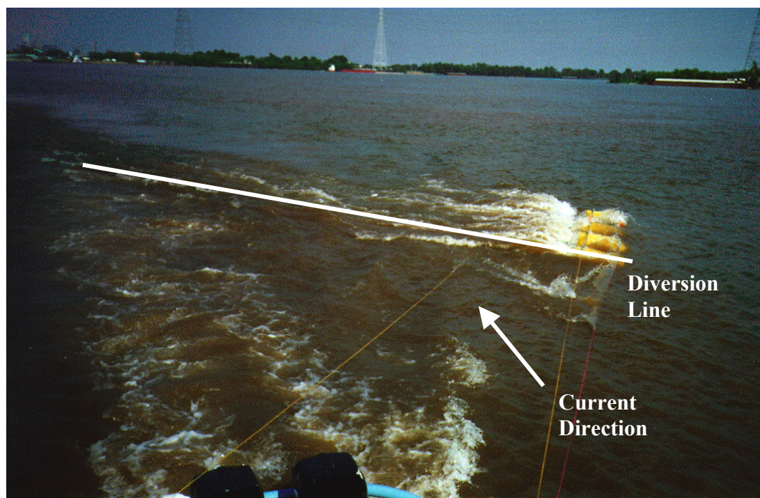
Figure 8. Diverter Catamarans Towed into Current (6 knots relative current)
