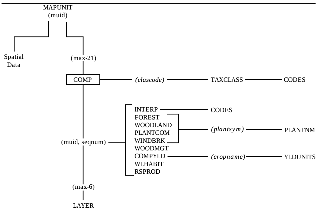
Figure 2. STATSGO table relationships
