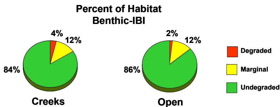
Figure 3.4.5. Estimates of the percent of the state's coastal habitat representing various Benthic IBI values that represent undegraded ( > 2.5 ), marginally degraded ( \geq 2 and \leq 2.5 ) or degraded ( < 2 ) benthic communities as developed by Van Dolah et al. (1999).
