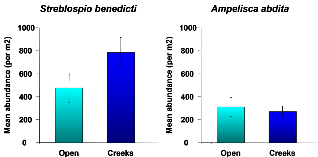
Figure 3.4.3. Abundance of two numerically dominant species, Streptospio benedicti and Ampelisca abdita , collected in benthic grabs at open water and tidal creek stations during 1999-2000.
