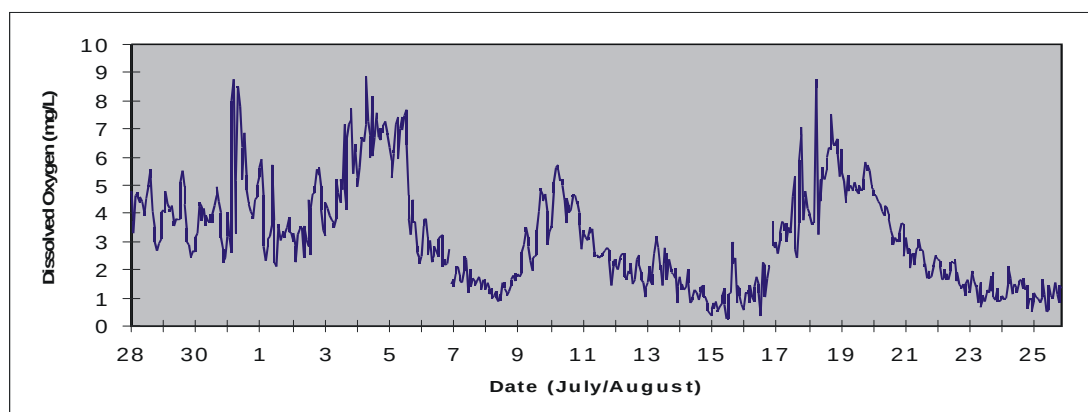
Figure 2-4. Continuous plot of bottom dissolved oxygen concentration at EMAP station 088 in Chesapeake Bay, 1990.
