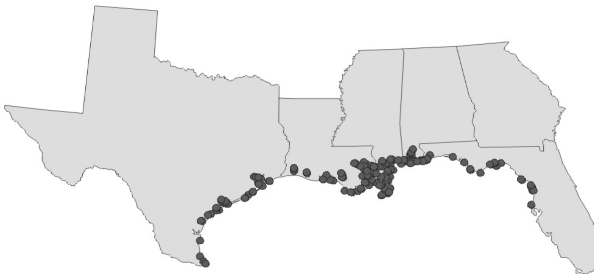
Figure 3-3. Map of EMAP-E sampling sites for 1991 in the Louisianian province.
