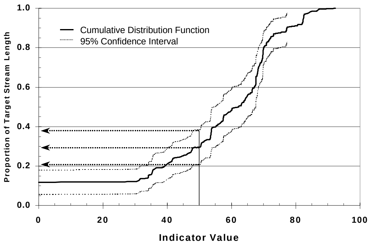
Figure 4-10. Hypothetical example showing how results from indicator values and monitoring framework will be used to estimate status of resource population.
