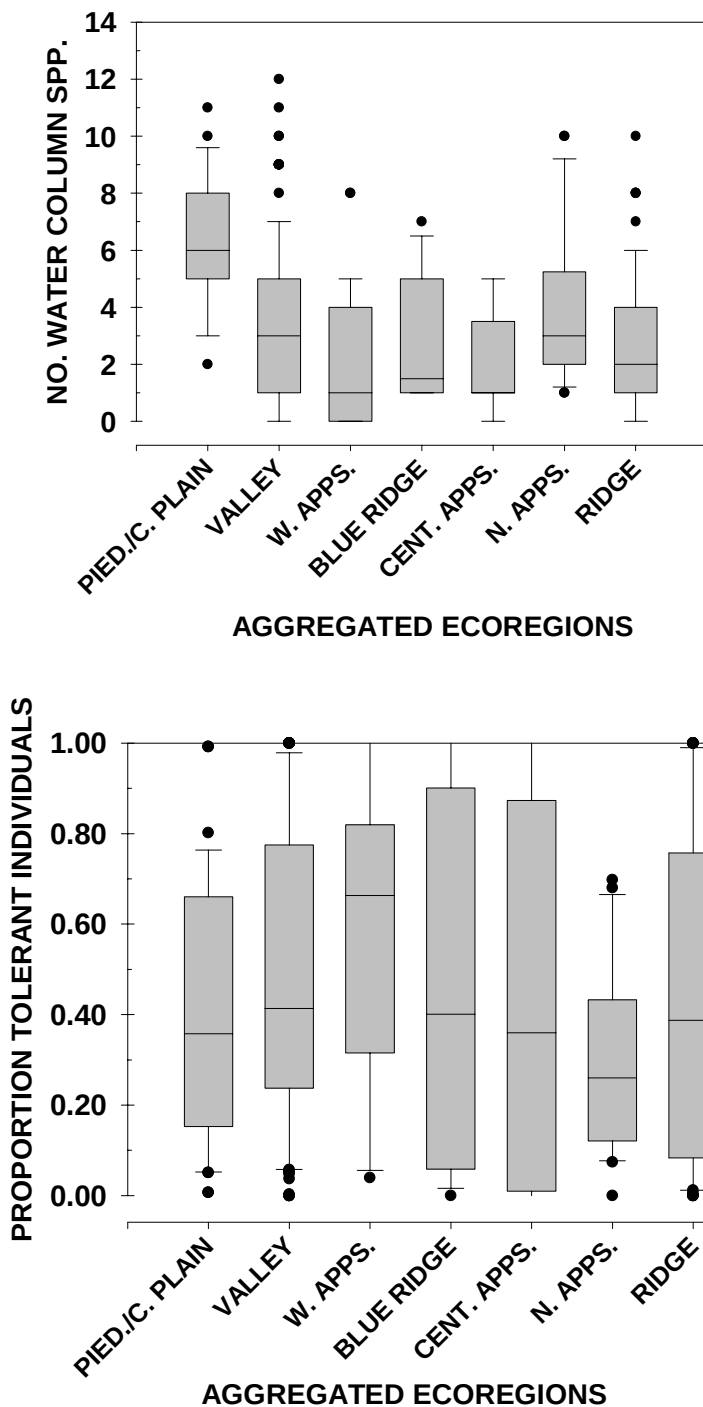
Figure 4-7. Examples of evaluating possible differences in metric expectations across MAHA subdivided by two levels of ecoregion aggregation. (A) number of water column species, a metric based on species richness; (B) proportion of individuals of tolerant species, a metric based on the proportion of individuals collected.
