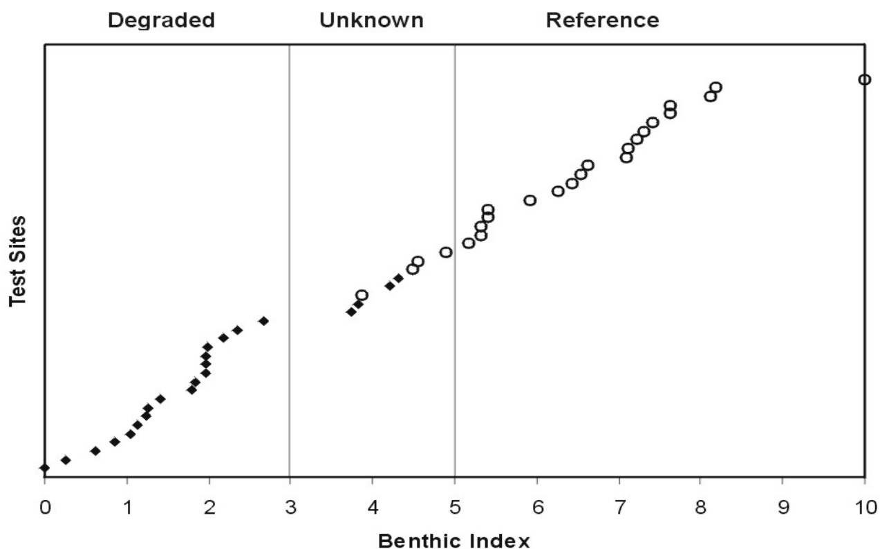
Figure 3-9. Distribution of benthic index values for the test sites where ◆ = degraded sites and ○ = undegraded sites determined by a priori criteria for dissolved oxygen, sediment chemistry, and sediment toxicity. The cutoff value for degraded sites determined by the benthic index is 3.0 and 5.0 is the cutoff value for undegraded sites determined by the benthic index.
