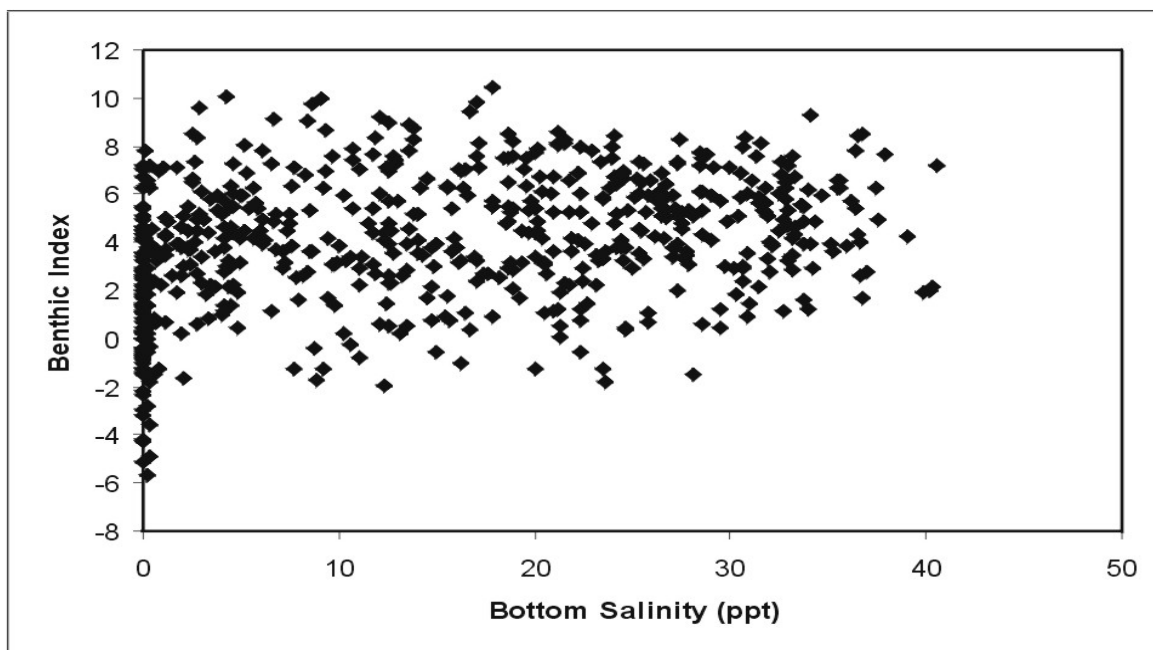
Figure 3-6. Benthic index versus bottom salinity for all sites from EMAP-E Louisianaian Province, 1991 to 1994.
