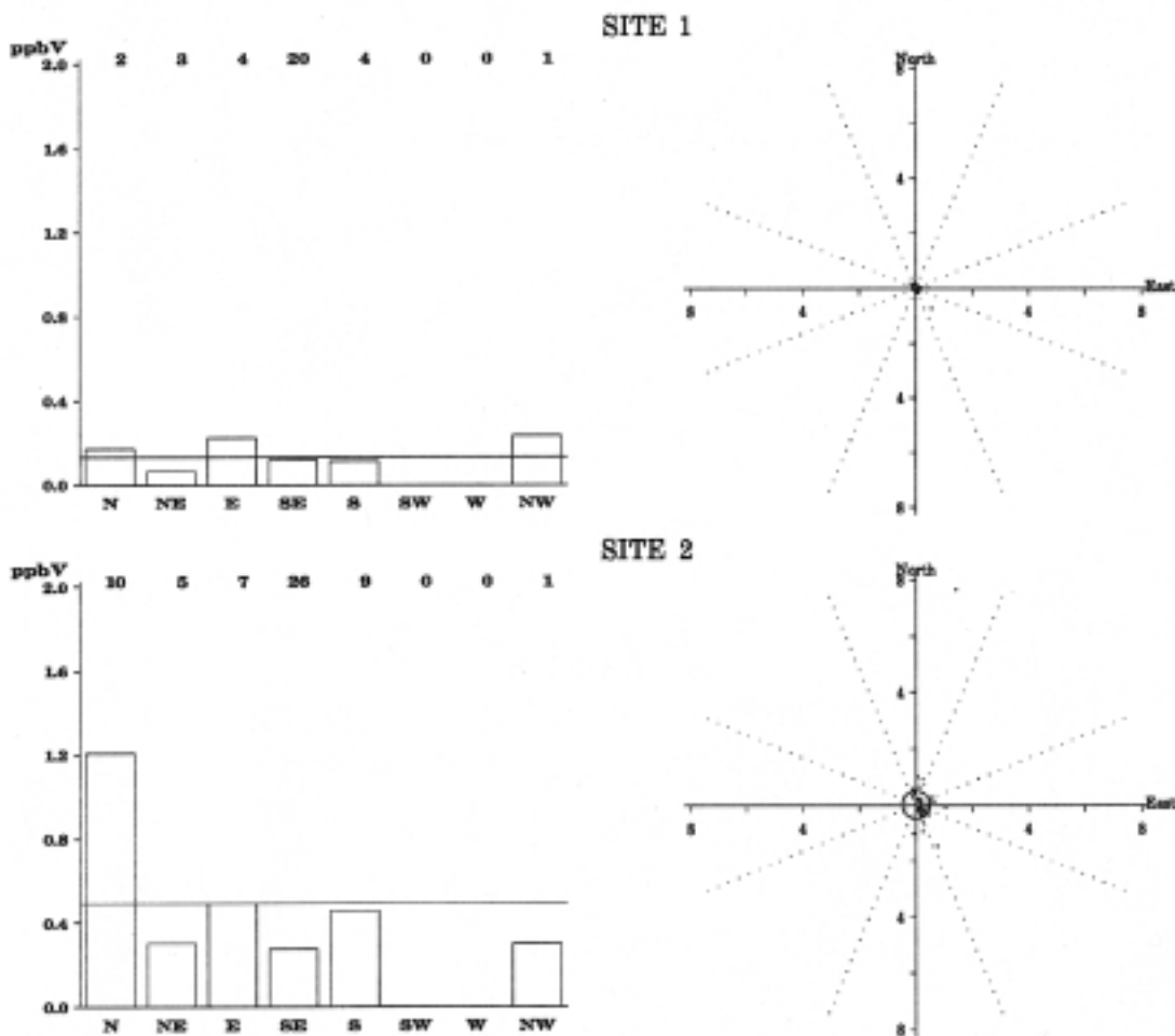
Figure 5.61. Bar charts and wind sector plots of o-Xylene concentrations (ppbV) at the three sites. See page 39 for a detailed explanation of figures.
