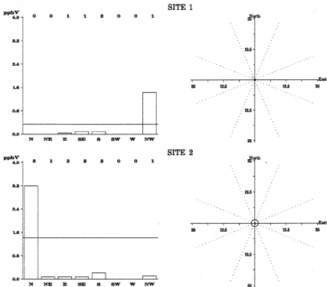
Figure 5.50. Bar charts and wind sector plots of Cyclohexane concentrations (ppbV) at the three sites. See page 39 for a detailed explanation of figures.
