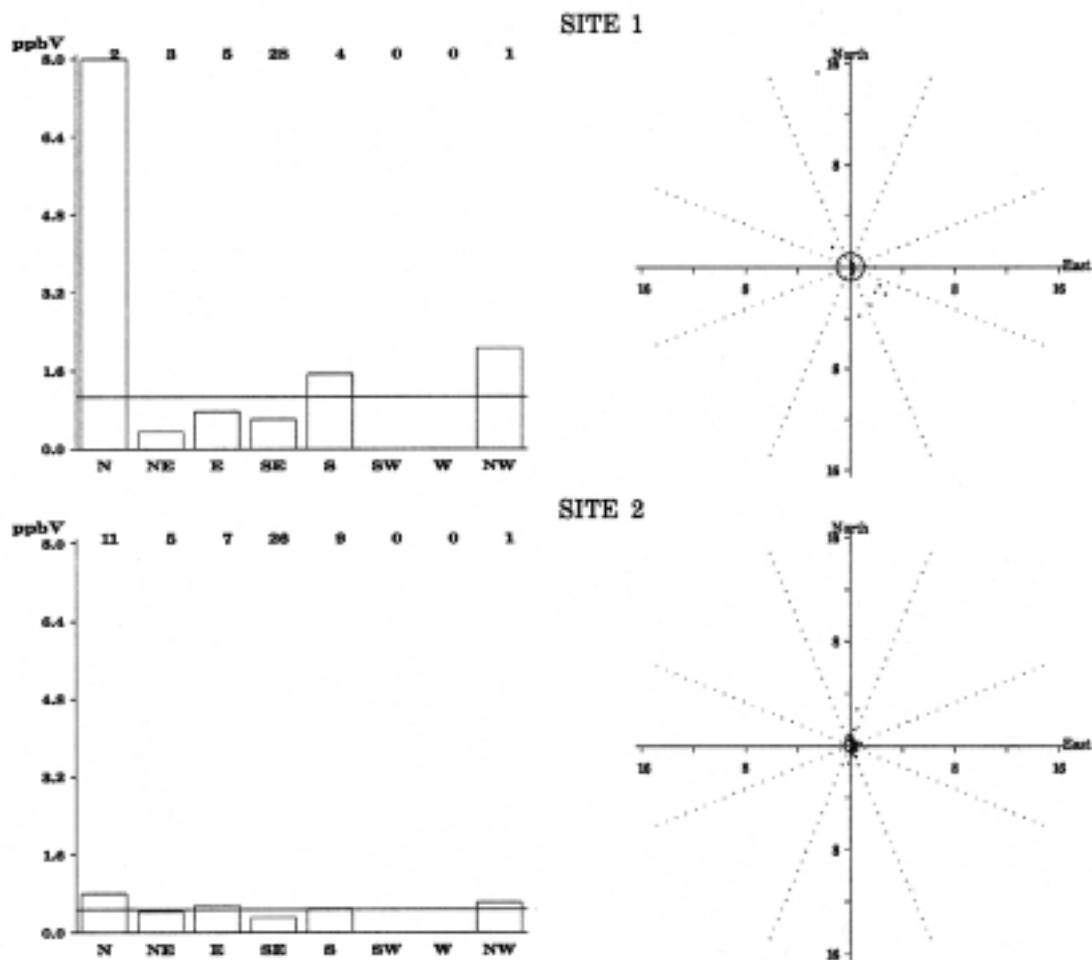
Figure 5.49. Bar charts and wind sector plots of Benzene concentrations (ppbV) at the three sites. See page 39 for a detailed explanation of figures.
