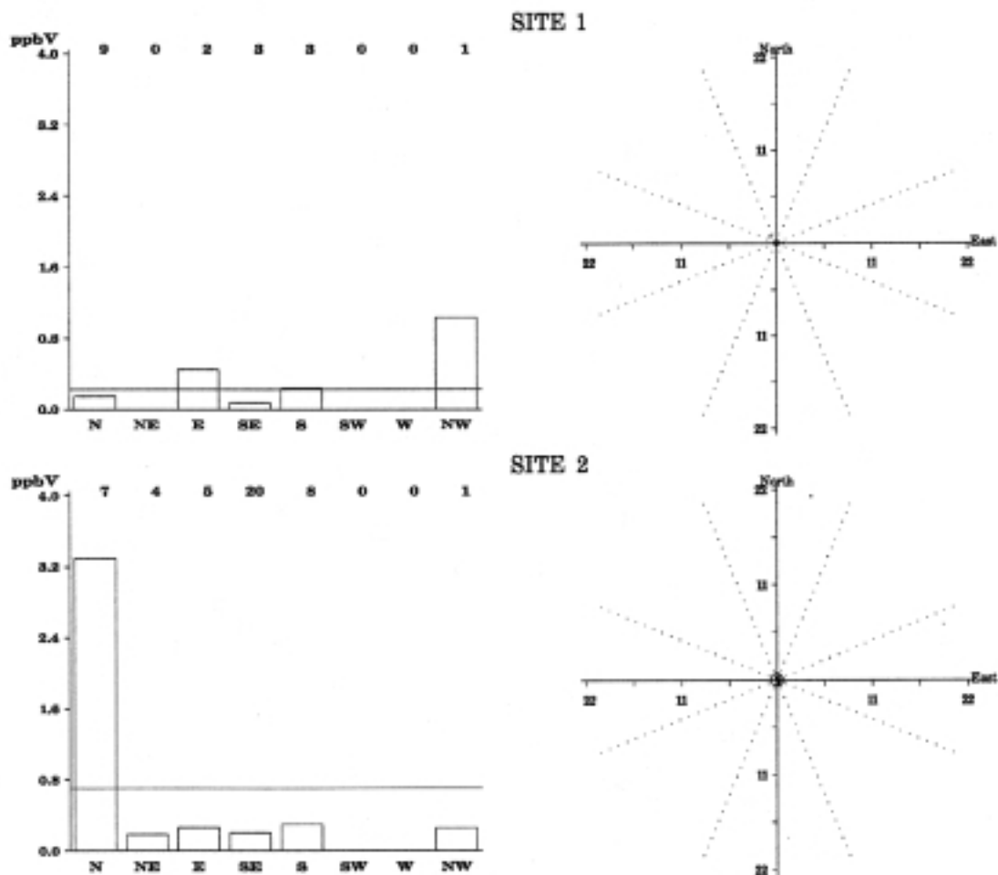
Figure 5.44. Bar charts and wind sector plots of 3-Methylhexane concentrations (ppbV) at the three sites. See page 39 for a detailed explanation of figures.
