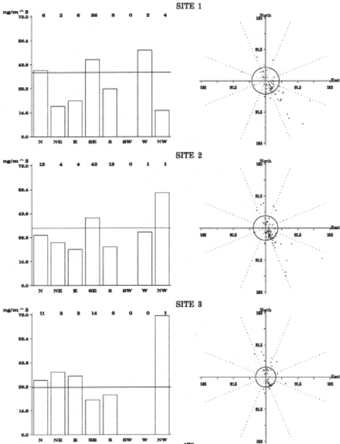
Figure 5.38. Bar charts and wind sector plots of coarse fraction Titanium (Ti) concentrations (ng/m 3 ) at the three sites. See page 39 for a detailed explanation of figures.
