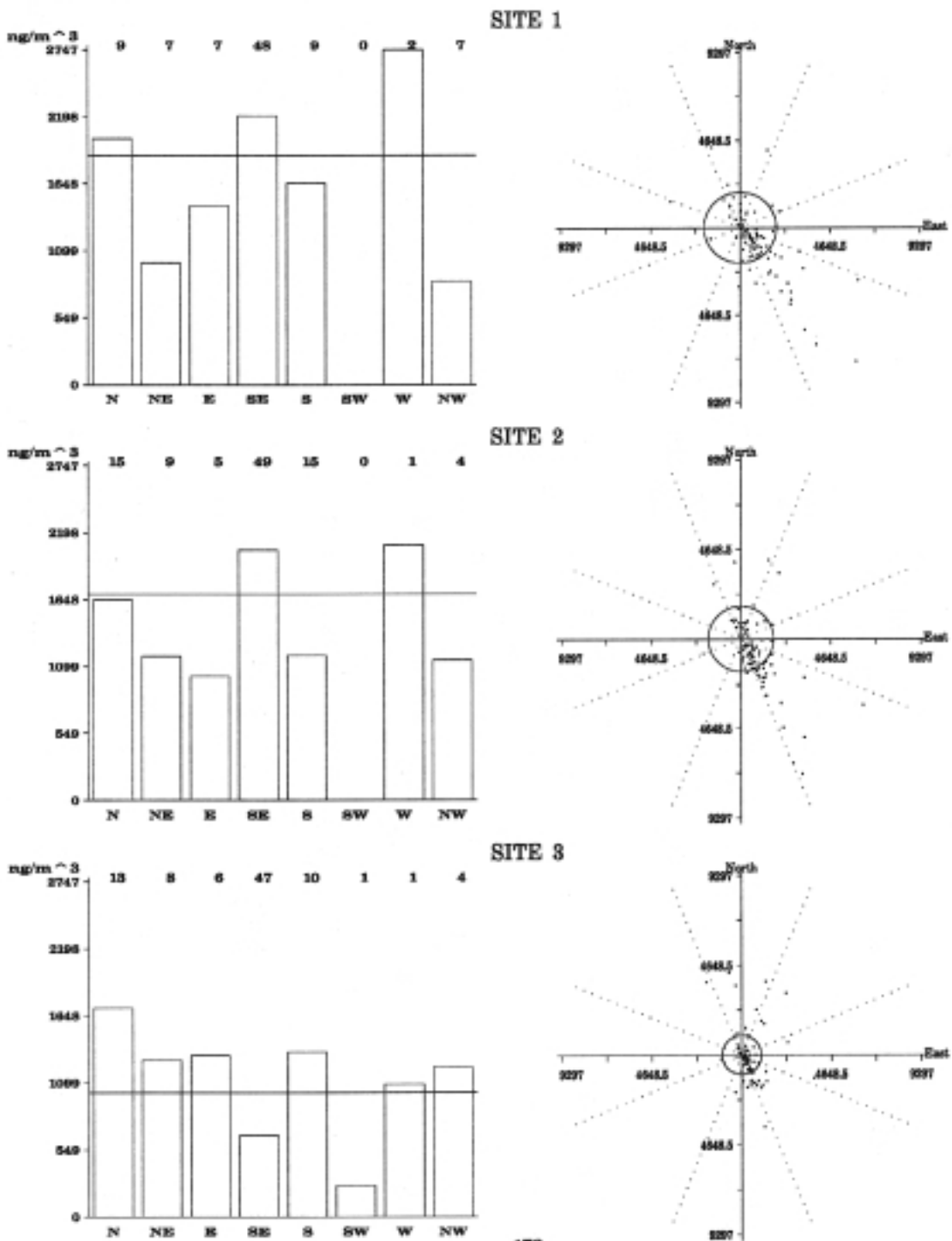
Figure 5.37. Bar charts and wind sector plots of coarse fraction Silicon (Si) concentrations ( \text{ng}/\text{m}^3 ) at the three sites. See page 39 for a detailed explanation of figures.
