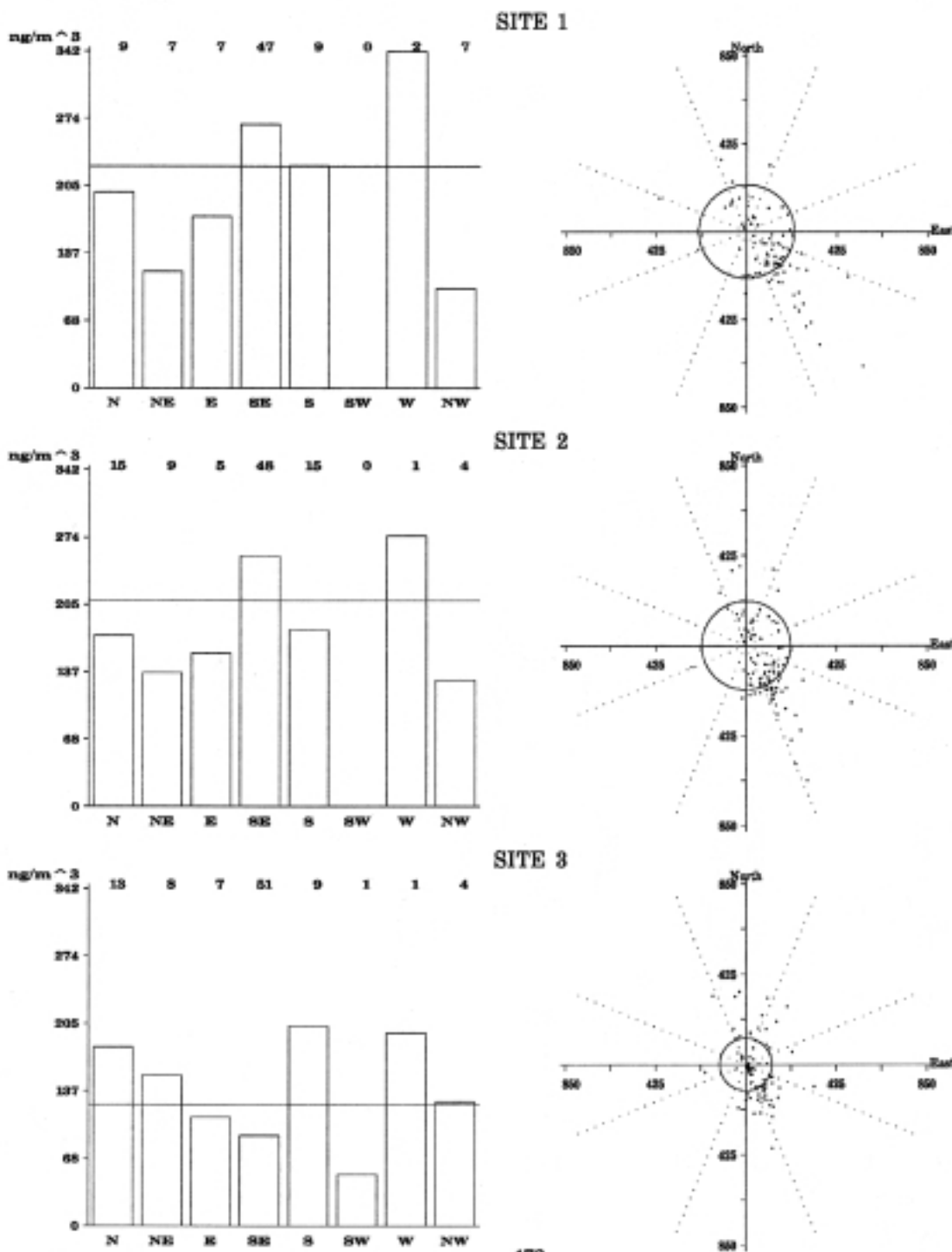
Figure 5.31. Bar charts and wind sector plots of coarse fraction Potassium (K) concentrations ( \text{ng}/\text{m}^3 ) at the three sites. See page 39 for a detailed explanation of figures.
