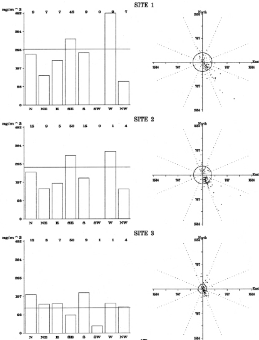
Figure 5.30. Bar charts and wind sector plots of coarse fraction Iron (Fe) concentrations ( \text{ng}/\text{m}^3 ) at the three sites. See page 39 for a detailed explanation of figures.
