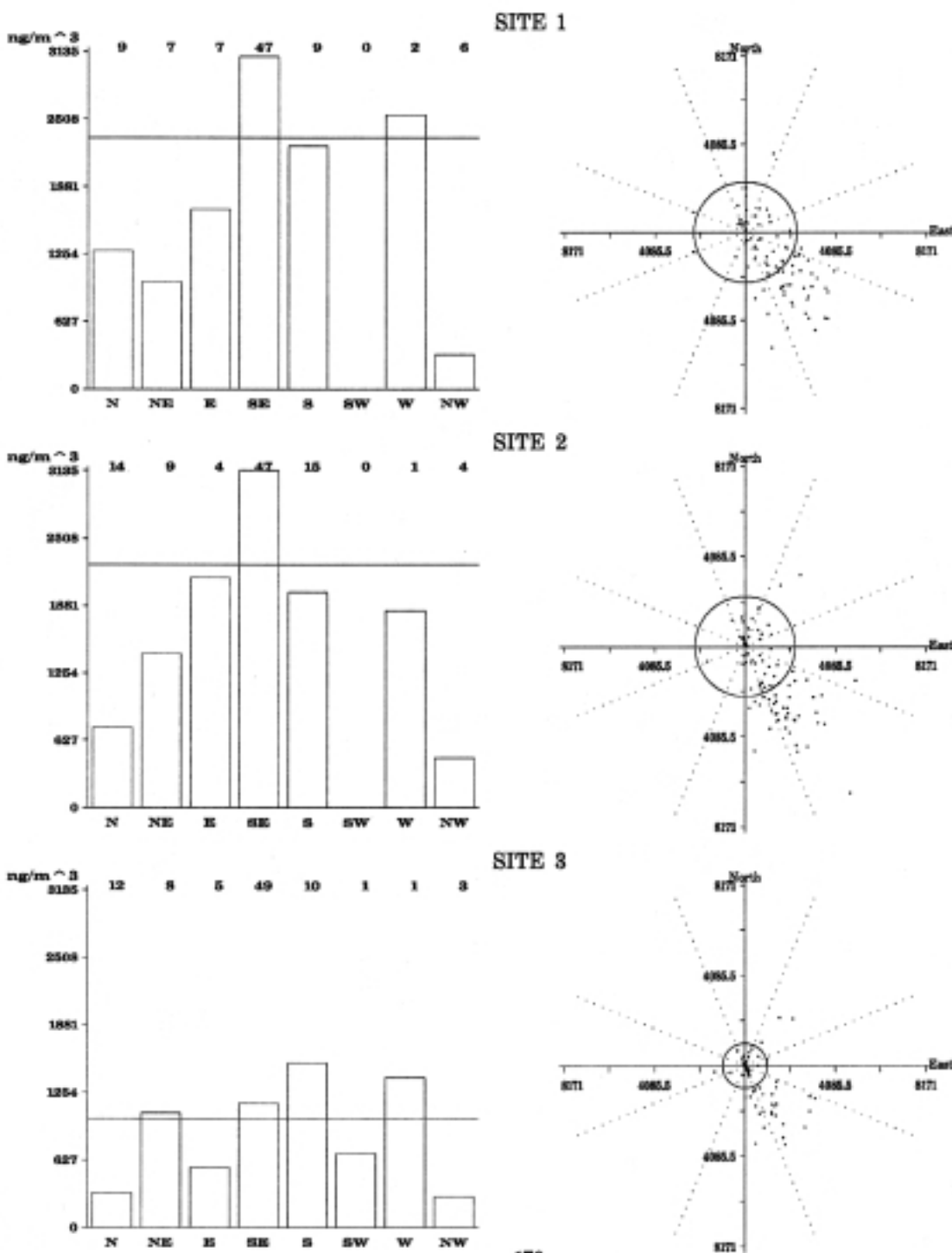
Figure 5.29. Bar charts and wind sector plots of coarse fraction Chlorine (Cl) concentrations ( \text{ng}/\text{m}^3 ) at the three sites. See page 39 for a detailed explanation of figures.
